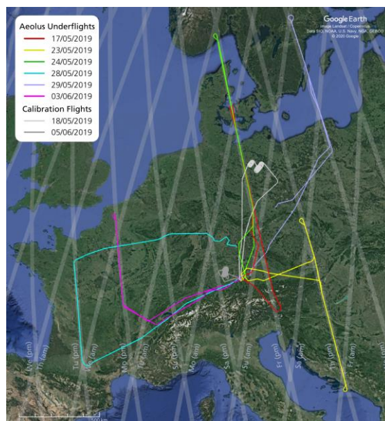
Figure 1. Flight tracks of the Falcon aircraft during the AVATARE campaign from 17 May to 5 June 2019 (background image: © 2020 Google). Each colour represents a single flight. The Aeolus measurement swath is shown in grey. The satellite flying direction was always from south to north during the probed evening ascending orbits.
