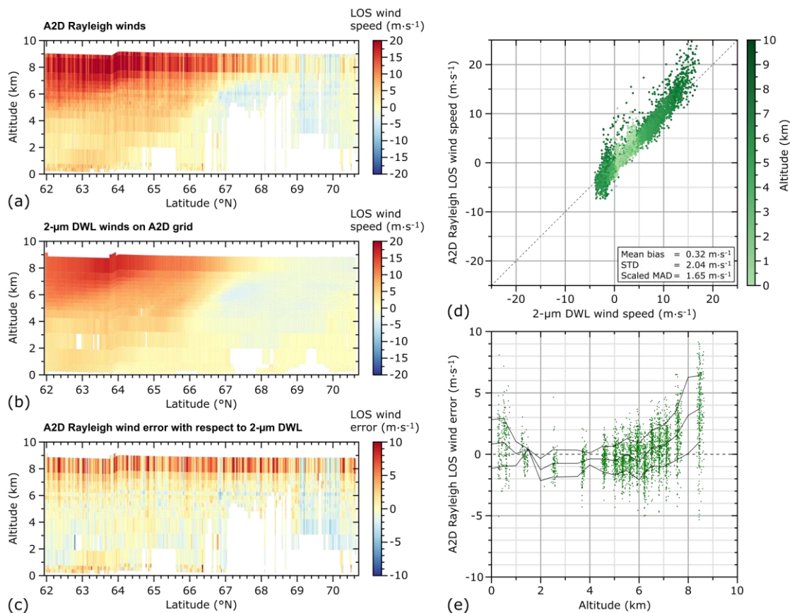
330 Figure 5. A2D Rayleigh wind for the AVATARI underflight on 16 September 2019 before the retrieval modifications: (a) A2D Rayleigh wind data, (b) 2- \mu m DWL wind data averaged onto the A2D measurement grid, (c) wind speed differences between (a) and (b), (d) scatterplots comparing the wind data from (a) and (b), where the color-coding describes the centre altitude of the considered range bin. Panel (e) depicts the altitude dependence of the A2D Rayleigh wind error with respect to the 2- \mu m DWL. The light green lines indicate the mean and standard deviation of the wind error in bins of 500 m.
