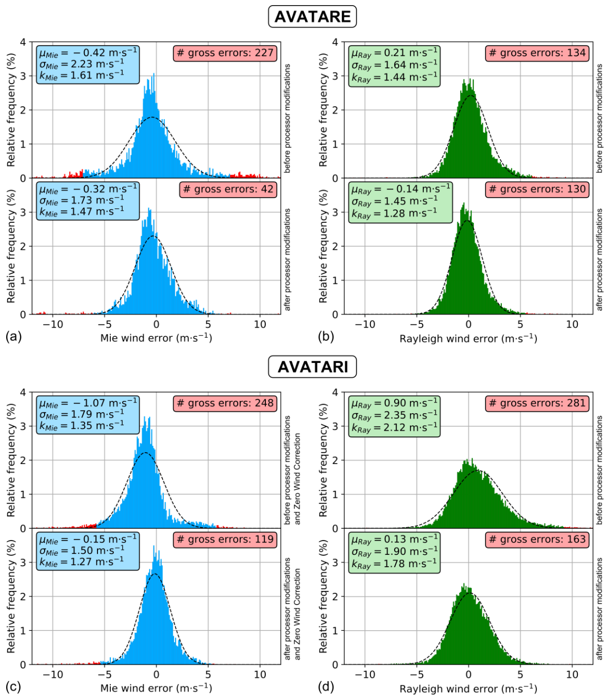
525 Figure 11. Probability density functions for the A2D Mie (a) and Rayleigh (b) wind error with respect to the 2- \mu m DWL for the entire AVATARE campaign before (top plot in each panel) and after (bottom plot) the applied retrieval modifications. Gross errors (see definition in the text) are marked in red. The dashed lines represent Gaussian fits. The insets summarize the mean values \mu , standard deviations \sigma and scaled MAD k calculated for the respective datasets. The corresponding PDFs of the A2D Mie and Rayleigh wind error for the AVATARI dataset are provided in panels (c) and (d), respectively.
