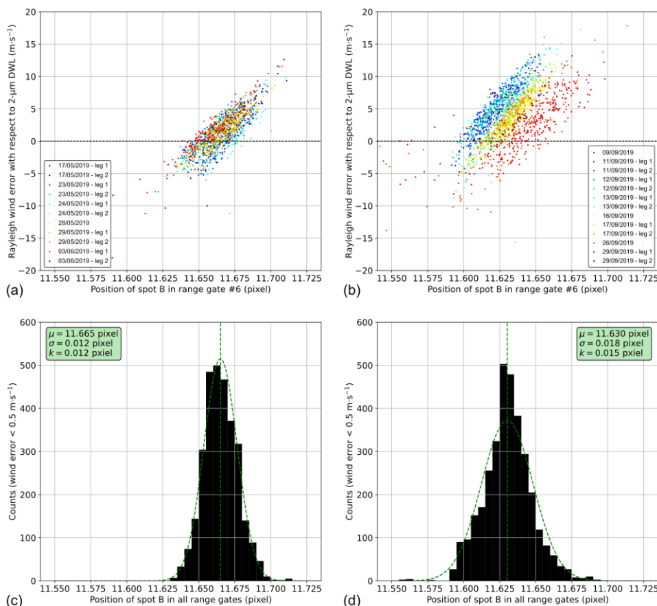
370 Figure 7. A2D Rayleigh wind error with respect to the 2- \mu\text{m} DWL in dependence on the position of spot B in range gate #6 for (a) the entire AVATARE campaign and (b) the entire AVATARI campaign (except for the underflights on 22/09/2019 and 23/09/2019). The scatters are color-coded according to the different Aeolus underflight legs. The bottom plots show histograms of spot positions from all range gates for which the wind error is \leq \pm 0.5 \text{ m}\cdot\text{s}^{-1} (bin size: 0.005 pixel).
