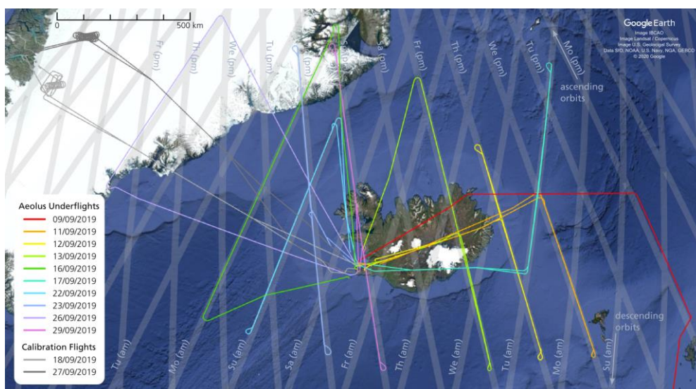
Figure 2. Flight tracks of the Falcon aircraft during the AVATARI campaign from 9 September to 29 September 2019 (background image: © 2020 Google). Each colour represents a single satellite underflight. The Aeolus measurement swath is shown in grey.
