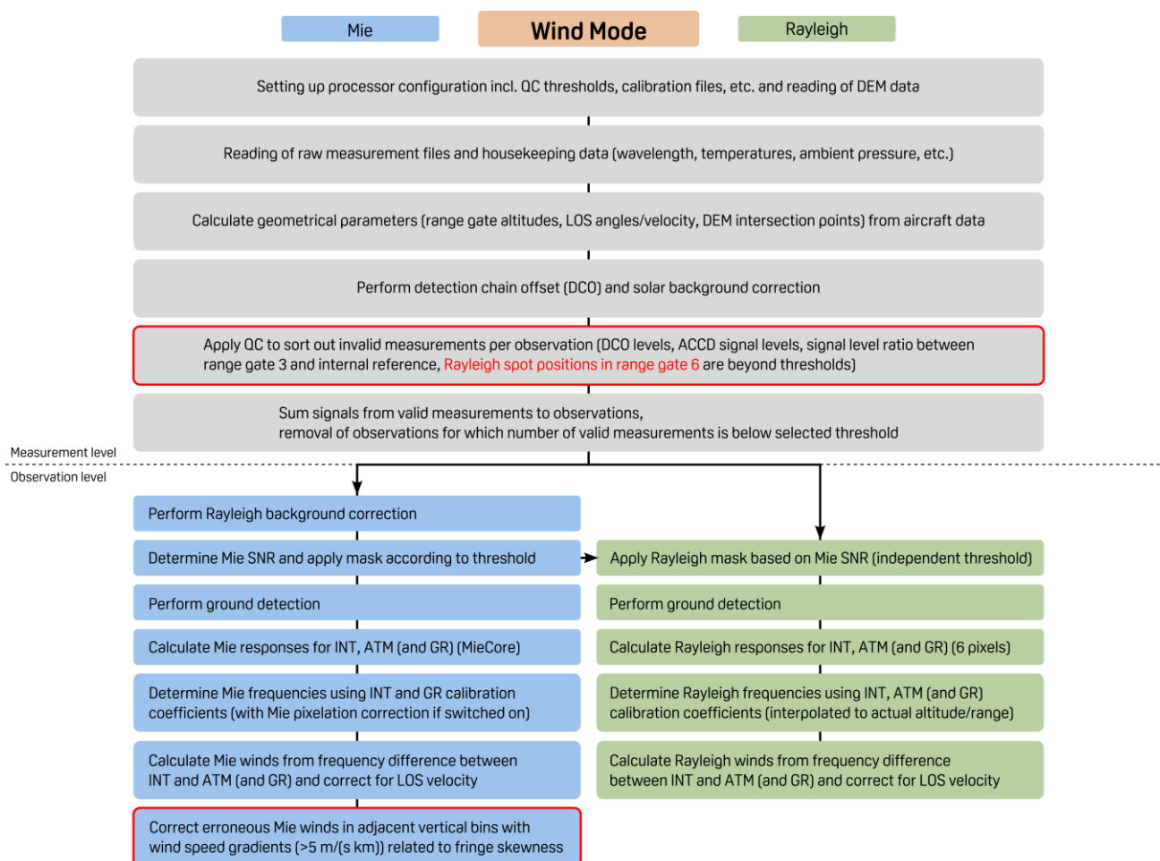
300 Figure 4. Flow chart of the A2D wind retrieval. Refinements that were introduced in the course of the AVATARE and AVATARI data analysis are indicated as red-framed boxes. INT: internal path; ATM: atmospheric path; GR: ground return.
