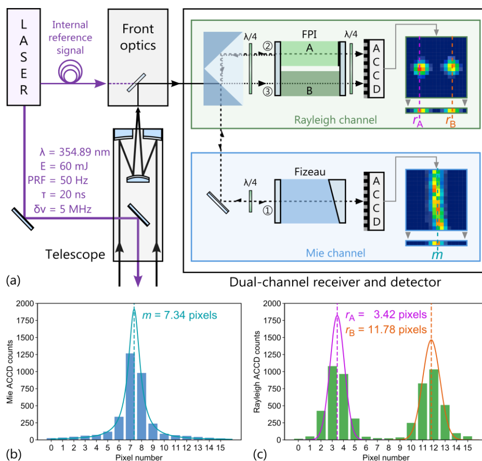
185 Figure 3. (a) Simplified schematic of the A2D comprising a frequency-stabilized, UV laser transmitter, a Cassegrain telescope, front optics and a dual-channel receiver. FPI: Fabry–Pérot interferometer; PRF pulse repetition frequency; ACCD: accumulation charge-coupled device. (b) Exemplary signal distribution measured with the Mie ACCD detector (blue bars) and Lorentzian fit of the signals transmitted through the FI for determining the Mie fringe centroid position m . (c) Exemplary signal distribution measured with the Rayleigh ACCD detector (green bars) and Gaussian fits of the signals transmitted through the two FPIs (A: pink, B: orange) for determining the Rayleigh spot positions 190 r_A and r_B .
