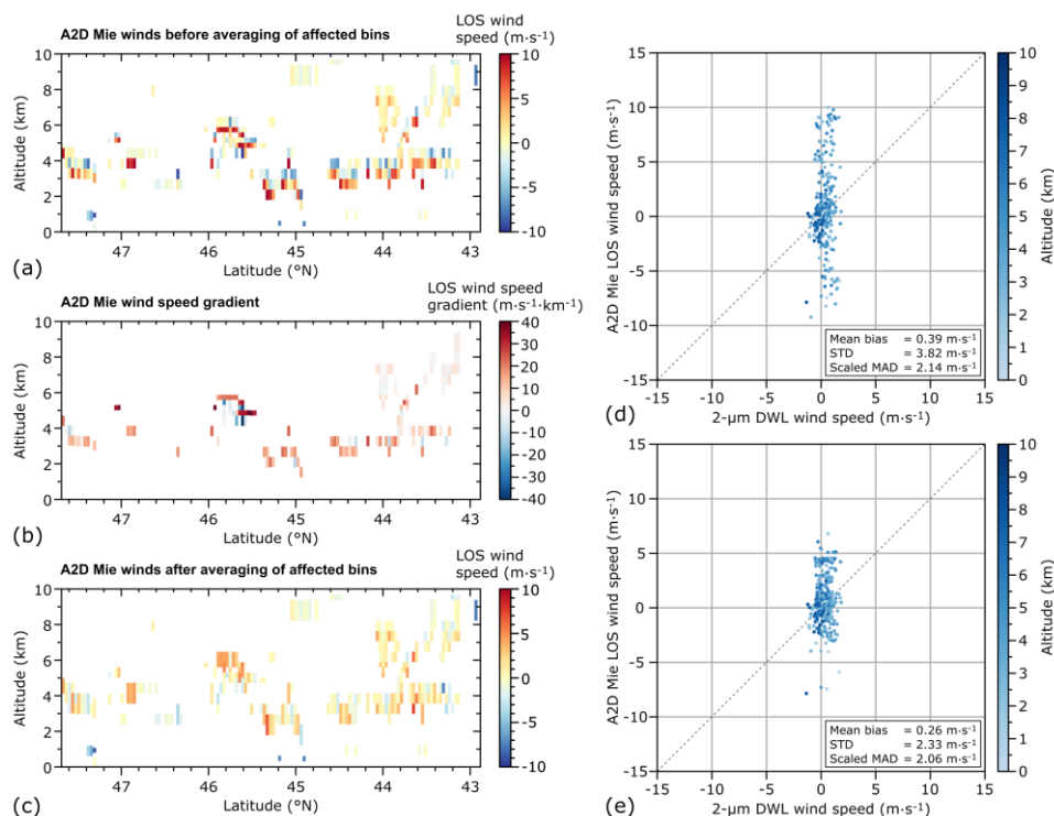
475 Figure 10. Mie winds for the AVATARE underflight on 23 May 2019 before and after retrieval modifications: (a) A2D Mie winds without bin averaging, (b) Mie wind gradient without bin averaging, (c) Mie winds with bin averaging. The right scatterplots show the correlation between the Mie winds and the 2- \mu m DWL wind data without (d) and with (e) bin averaging.
