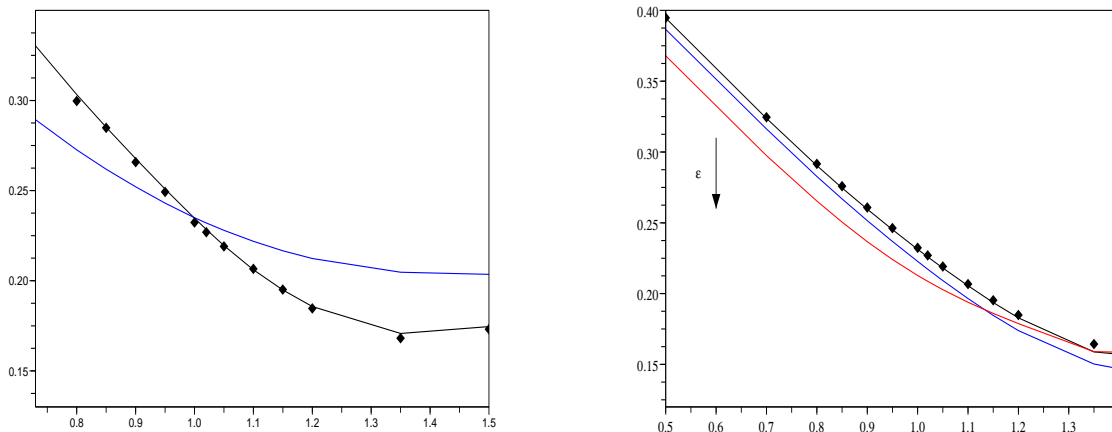
Figure 3: Left: diamonds indicate market 1 year implied volatility for the DAX. The curve fitting this data is the implied volatility given by the local correlation model (57) with \gamma = 8.672568 , \eta = 0.500714 and \rho_{\min} = 0.1 . The other curve is the implied volatility given by a constant correlation model (C_t)_{i,j} = \mathbb{1}_{i=j} + \rho \mathbb{1}_{i \neq j} that fits the at the money implied volatility: \rho = 0.67968 . Right: With the same values for \gamma , \eta and \rho_{\min} , we have plotted for \kappa = 100 and \varepsilon \in \{0, 0.3, 0.9\} the implied volatility given by model (58). These curves are obtained with 10^6 Monte-Carlo samples and discretization time step 0.025.
