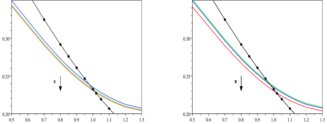
Figure 2: In both graphics, the line with diamonds indicate the market 1 year implied volatility. We plot the implied given by model (56) with \rho = 0.67968 and use the parametrization a = \sqrt{\frac{2\kappa\varepsilon}{d-1}(1-\rho)} , with \varepsilon \in [0, 1] . Left: \kappa = 100 and \varepsilon \in \{0, 0.6, 1\} . Right: \varepsilon = 0.5 and \kappa \in \{1, 20, 100\} . These curves are obtained with 10^6 Monte-Carlo samples and discretization time step 0.025.
