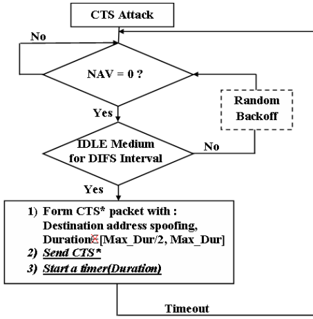
Fig. 3. The false CTS flow chart
