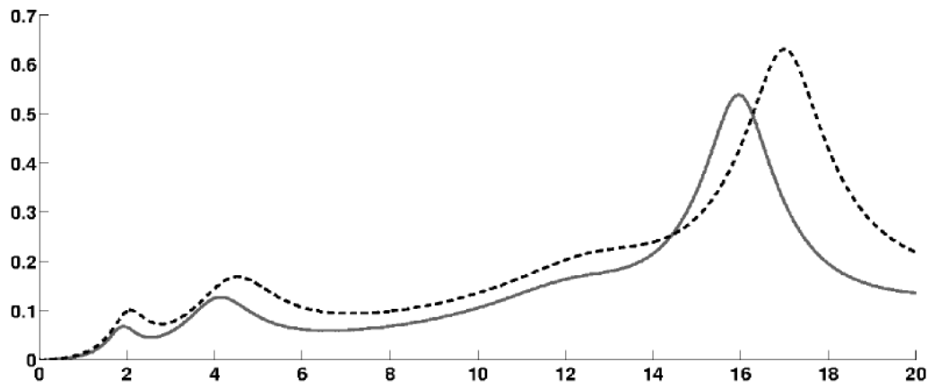
Fig. 4 Graph of the dynamic magnification factor function for the beam models with homogeneous mass (solid line) and the lumped mass model (dashed line). Horizontal axis \omega in Hz. Vertical axis: dynamic magnification factor H(\omega)
