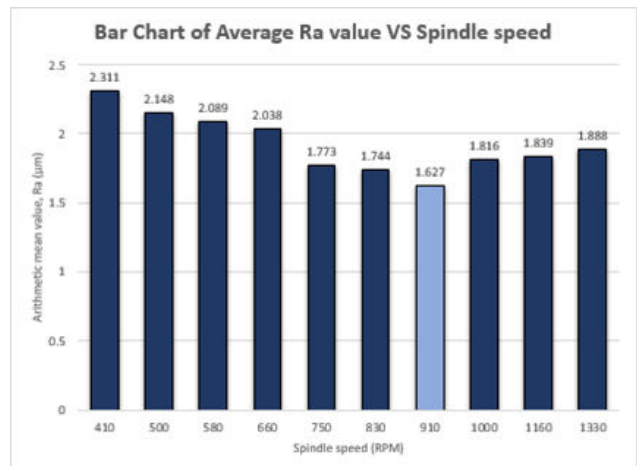
Figure-3.1. Bar chart of comparison between the arithmetic means value and spindle speed.
