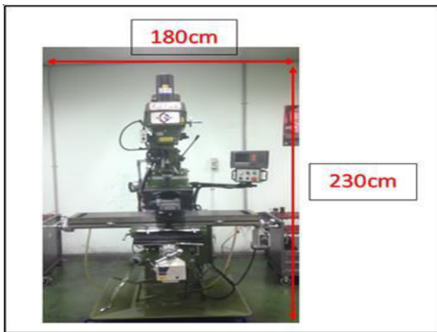
Figure-2.2. Vertical milling machine.
