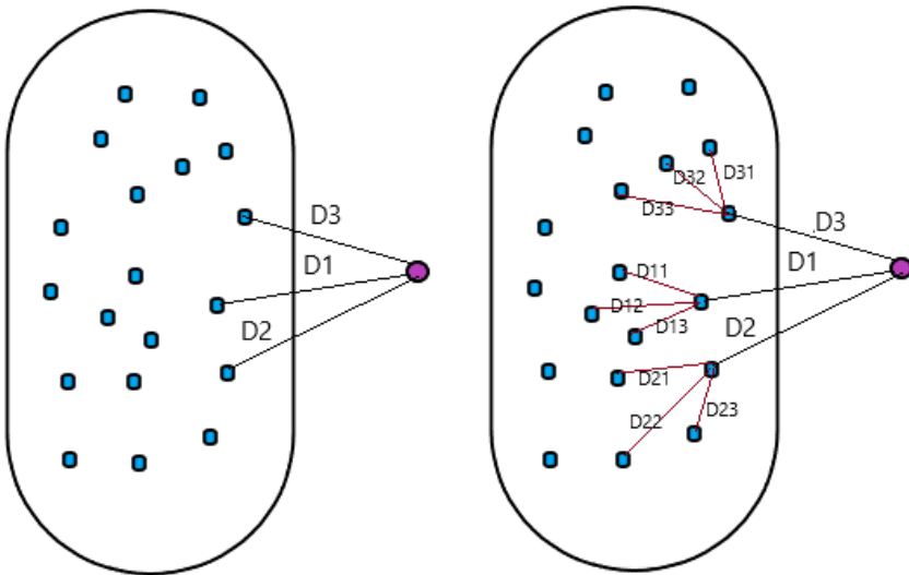
Figure 1. k -NN (left) and jk -NN (right)
