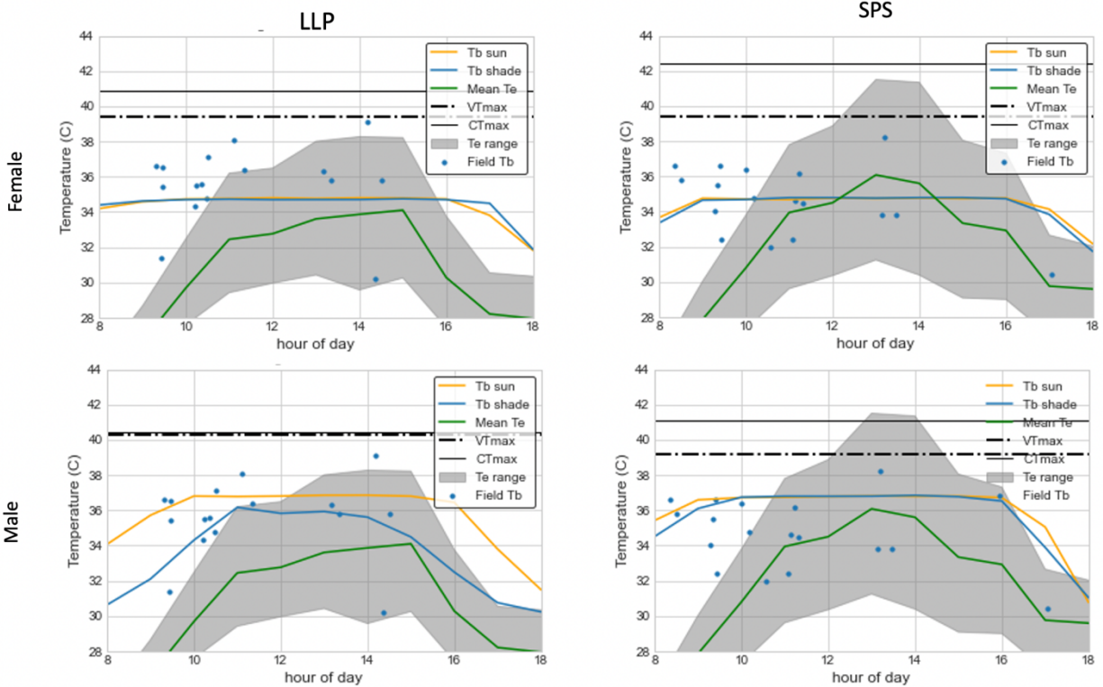
Figure 4: Top left and top right panels depict female data in LLP and SPS habitats respectively. Bottom left and right panels depict male data in LLP and SPS respectively. Solid and dotted black lines and blue dots depict empirical thermal preference data; shaded gray area depicts operative temperature range recorded by iButton dataloggers; blue and yellow lines depict NicheMapR predicted body temperatures in sunny and shady environments. Recorded operative temperatures do not reach CTmax for any sex except males in SPS habitats. NicheMapR predicted body temperatures fall within empirical field-active Tb range for females; empirical male field active Tb tended to be lower than NicheMapR predicted body temperature.
