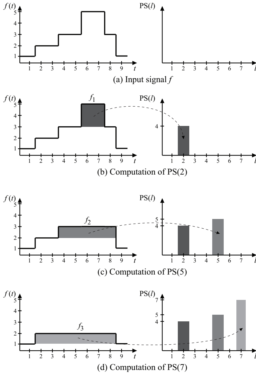
Figure 2.7: Example of 1-D signal f and creation of the pattern spectrum PS(l) .
