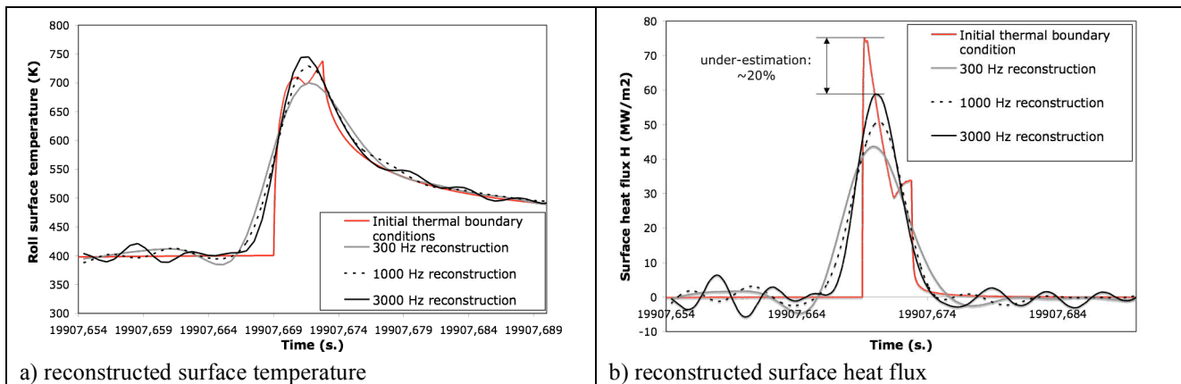
Fig. 3: zoom in the roll bite area (last roll rotation of coil n°56: Evaluation by direct/inverse simulation of reconstructed roll surface temperature and reconstructed heat flux for 3 acquisition frequencies for the sub-surface temperature (distance: 0.48 mm)
