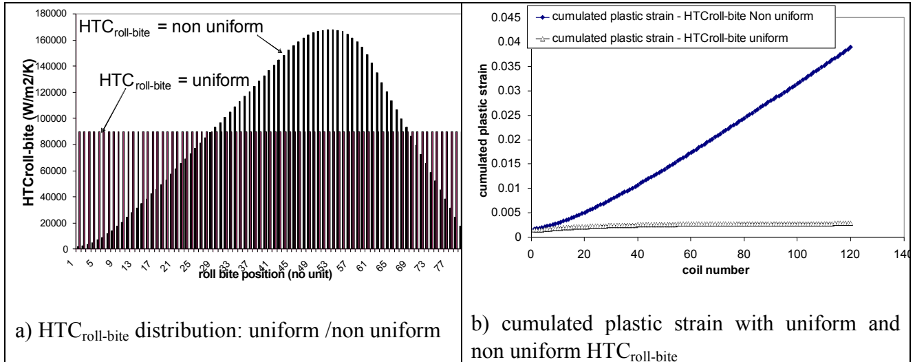
Fig.15: respective influence of uniform and non-uniform HTC_{roll-bite} (a) on roll thermal fatigue degradation (b). (Industrial rolling conditions used are in §3)
