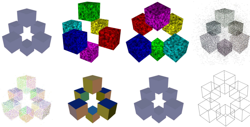
Figure 7.10: cubes data set : a simple model, samples synthetic images, point cloud from interest points, segmented point cloud and concise piecewise-planar reconstruction (colored by plane / wireframe contours).
