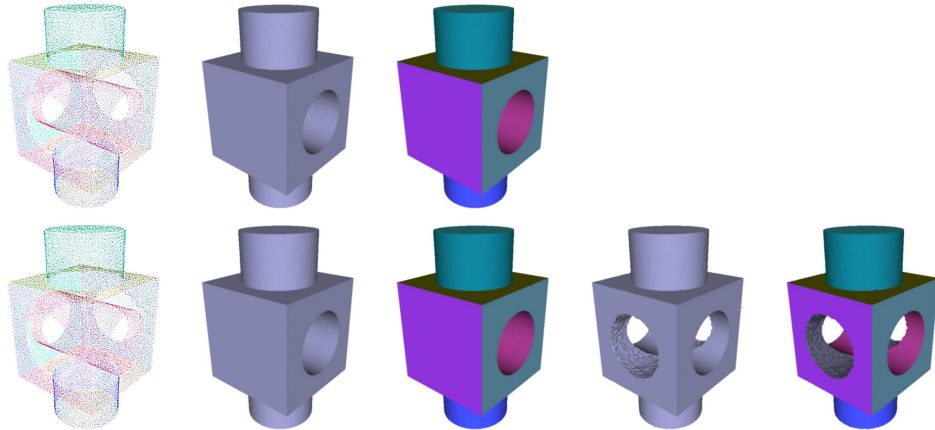
Figure 8.4: block data set . First row: shape extraction result with one of the detected shape purposely removed and shape-based reconstruction result. Second row: hybrid reconstruction result with a high \lambda_{\text{qual}} and hybrid reconstruction result with a low \lambda_{\text{qual}} .
