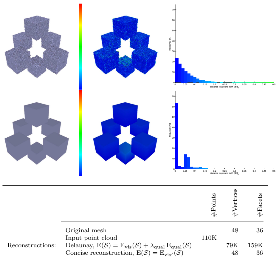
Figure 7.11: cubes data set : comparison with the generic reconstruction method of Chapter 3 (the normal estimate and outliers level were too high for Poisson to succeed). First row: Delaunay, second row: concise piecewise-planar reconstruction. First column: reconstructed surface, second column: reconstructed surface (colored by distance to ground truth), third column: histogram of distances to ground truth.
