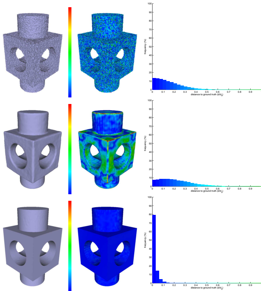
Figure 8.7: block data set : comparison with the general purpose reconstruction methods of Chapter 4 and Poisson surface reconstruction. First row: Delaunay, second row: Poisson, third row: our shape-based reconstruction. First column: reconstructed surface, second column: reconstructed surface (colored by distance to ground truth), third column: histogram of distance to ground truth.
