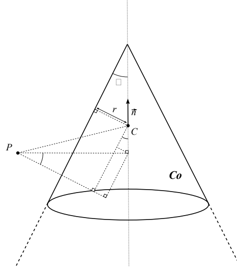
Figure A.4: A cone Co_{\vec{n}, d} , the geometric meaning of its parameters and a point P .
