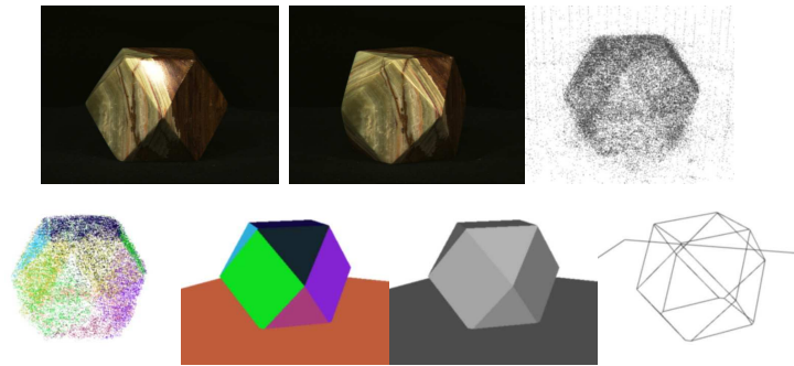
Figure 7.13: ALOI #418 data set : two of the 72 input images, input point cloud, segmented point cloud and concise piecewise-planar reconstruction (colored by plane / uncolored / wireframe contours).
