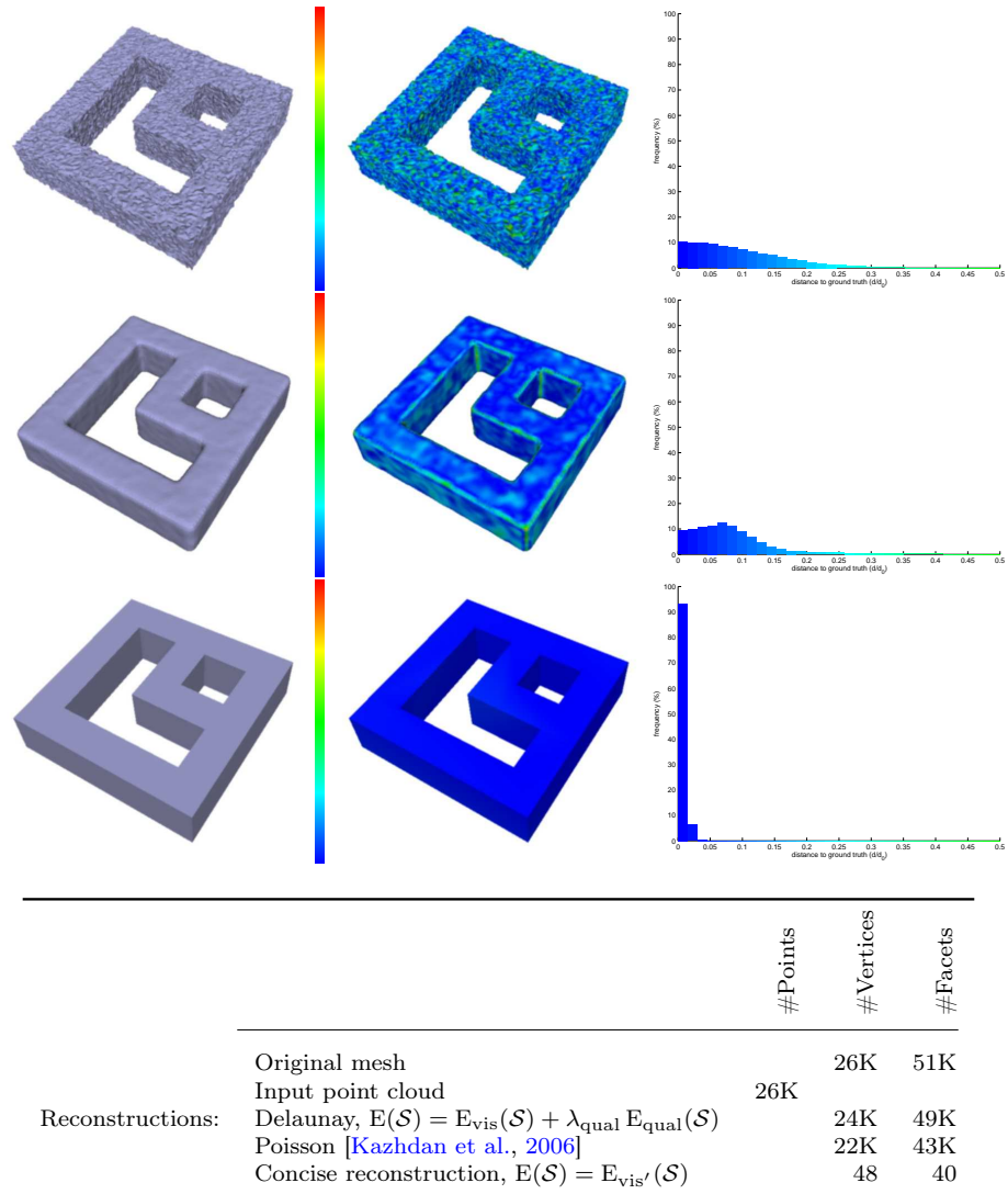
Figure 7.6: double torus II data set : comparison with the general purpose reconstruction method of Chapter 3 and Poisson surface reconstruction. First row: Delaunay, second row: Poisson, third row: concise reconstruction. First column: reconstructed surface, second column: reconstructed surface (colored by distance to ground truth), third column: histogram of distances to ground truth.
