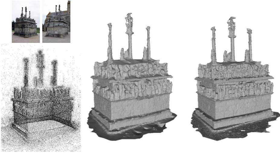
Figure 4.5: calvary data set . From left to right: two of the 27 images (8 Mpix) of a sculpted calvary taken from the ground, the generated point cloud (1,300,000 points), the initial mesh \mathcal{S}^0 (1,200,000 triangles) and the final reconstruction (1,850,000 triangles).
