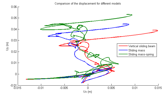
FIGURE 5. Seismic loading - Comparison of models
