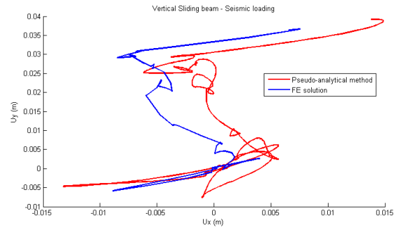
FIGURE 4. Vertical Sliding Beam - Seismic loading - Displacement curves
