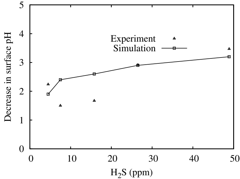
Figure 2.4: Decrease in surface pH ( pH_{(initial)} - pH_{(exposed)} ) after 1 year.
