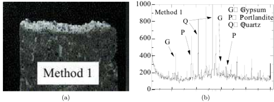
Figure 6.1: After 90 days immersion test: (a) Observation of deterioration of sample; (b) XRD patterns of surface area of sample. (Method 1, pH = 1) (Kawai et al., 2005)
