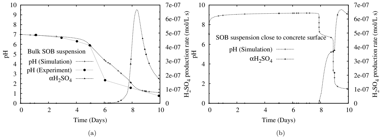
Figure 7.13: The pH evolution and production rate of H_2SO_4 from 0 to 10 days: (a) bulk SOB suspension; (b) SOB closed to concrete surface.
