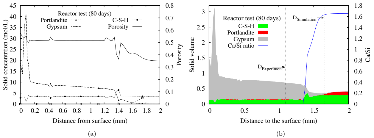
Figure 7.21: After 80 days of test in simulation reactor: (a) Solid concentration and porosity ; (b) Solid volume and Ca/Si ratio of C-S-H. ( H_2S level = 400 ppm)
