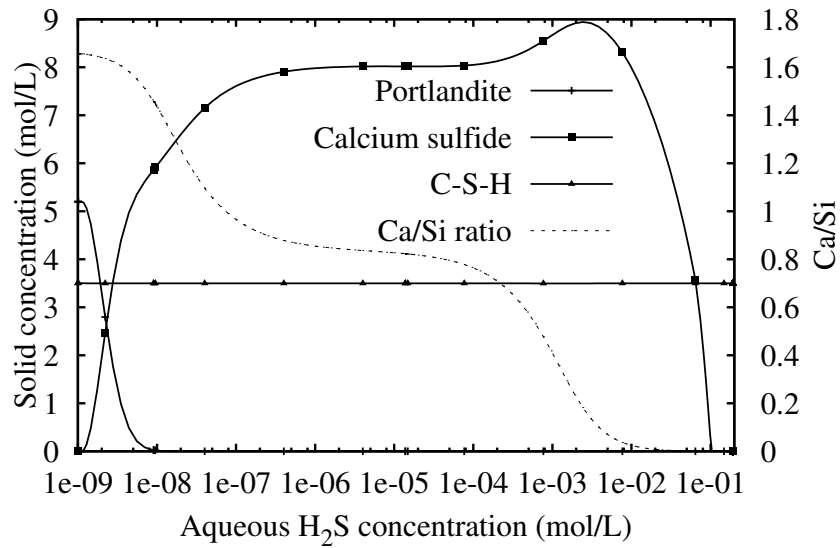
Figure 3.5: Evolution of the solid composition vs. H_2S concentration in REV of cement paste
