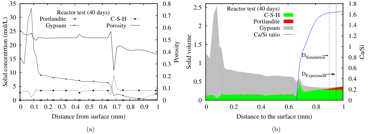
Figure 7.20: After 40 days of test in simulation reactor: (a) Solid concentration and porosity ; (b) Solid volume and Ca/Si ratio of C-S-H. ( H_2S level = 400 ppm)
