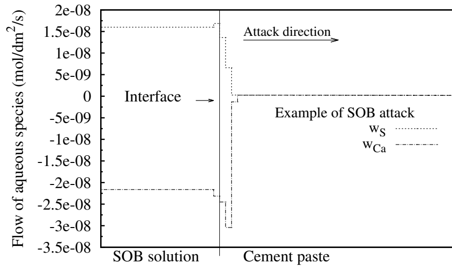
Figure 5.12: Flow of aqueous species across the interface at 1 day
