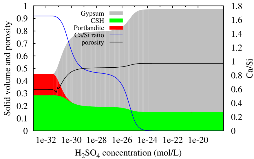
Figure 4.10: Evolution of the solid volume and porosity vs. H_2SO_4 concentration in REV of cement paste
