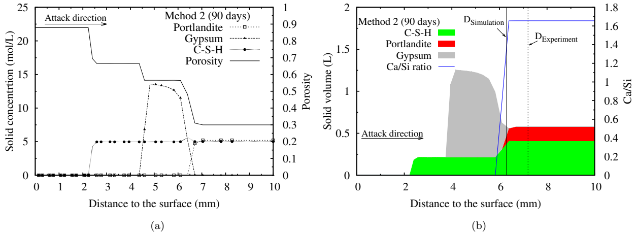
Figure 6.12: After 90 days of immersion: (a) Solid concentration and porosity ; (b) Solid volume and Ca/Si ratio of C-S-H . D_{\text{Simulation}} and D_{\text{Experiment}} represent the degradation depth of the sample in simulation and experiment individually. (Method 2, \text{pH} = 1 )
