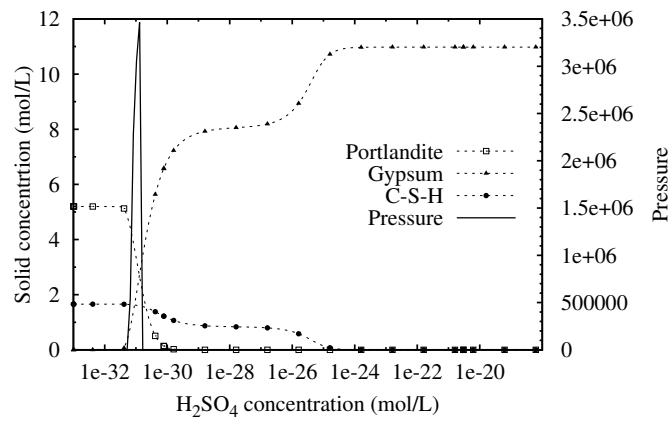
Figure 4.11: Evolution of inner pressure vs. content of CH and C\bar{S}H_2 in REV of cement paste
