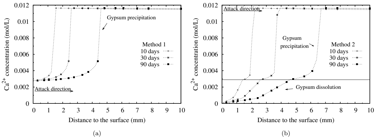
Figure 6.13: The calculated \text{Ca}^{2+} concentration profiles during immersion: (a) Method 1 ; (b) Method 2 . ( \text{pH} = 1 )
