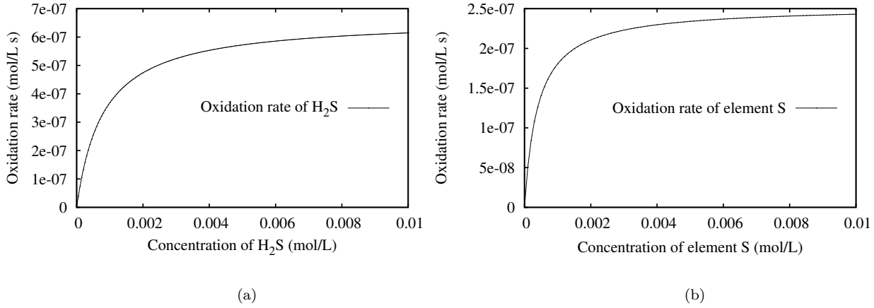
Figure 2.9: Oxidation rate : (a) H_2S ; (b) element S.
