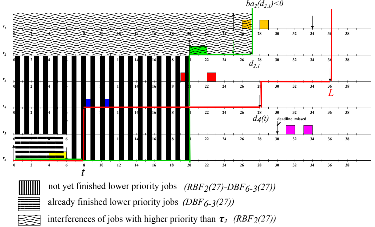
Figure 3: Energy balance of J_{2,1} at time t=8
