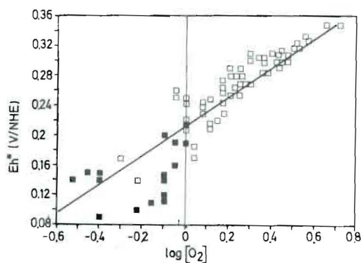
Fig. 9 : The Fontenay-Tresigny plant : potentials reached in situ at the end of the aeration periods against the logarithm of dissolved oxygen concentration (expressed in \text{mg O}_2 \cdot \text{l}^{-1} ).
