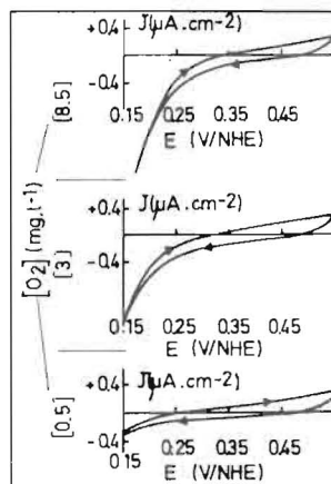
Fig. 2 : Voltammetric curves at different dissolved oxygen levels in activated sludge stationary electrode - platinum surface area : 0.5 \text{ cm}^{-2} - scan rate : 75 \text{ mV.min}^{-1}
