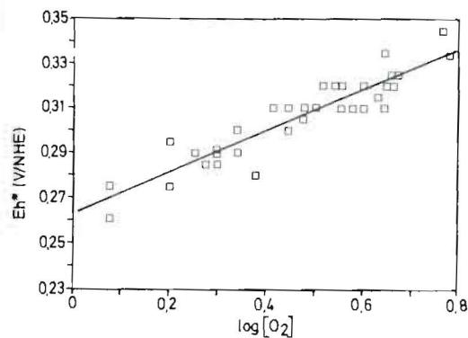
Fig. 8 : The Crisolles plant : potentials reached in situ at the end of the aeration periods against the logarithm of the dissolved oxygen concentration (expressed in \text{mg O}_2 \cdot \text{l}^{-1} )
