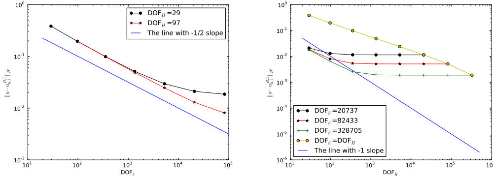
FIG. 5. Numerical errors \|u - u_{h,1}^{H,1}\|_{H^1} ( \mathbb{P}_1 finite elements), as functions of DOF_h (left) and DOF_H (right) (in log-log scale).
