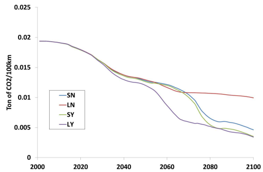
(d) Average private vehicle emissions per passenger-km. Average over all circulating private cars. Public transport emissions are much smaller, about 4.10^{-4} tCO 2 /100km or less in all scenarios.
