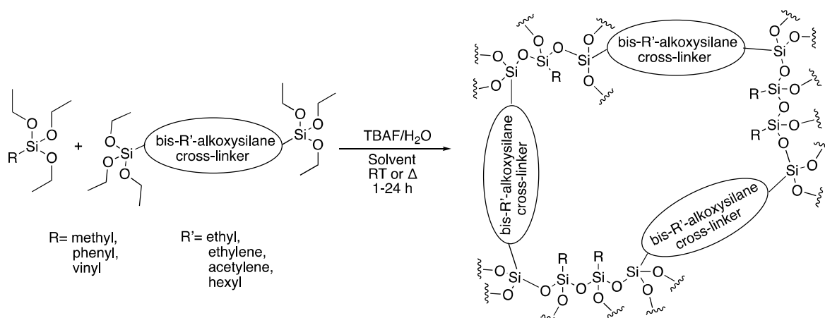
Scheme 1. Reaction to form silsesquioxane networks using fluoride-catalyzed synthesis. TBAF: tetrabutylammonium fluoride. *RT = room temperature.
