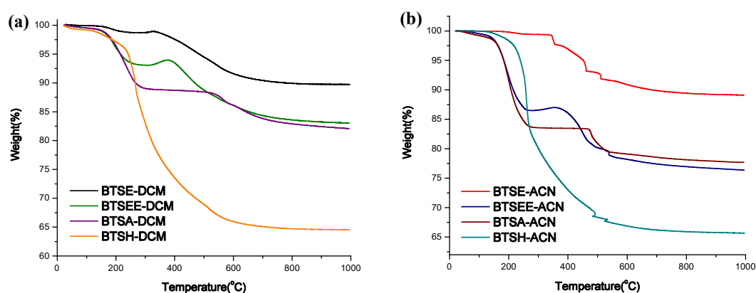
Figure 1. Thermal Gravimetric Analysis (TGA) graphs (in air) of materials from reactions with different cross-linkers in (a) dichloromethane and (b) acetonitrile, note BTSEE shows oxidation of the double bond at 400 °C.
