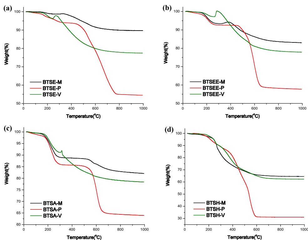
Figure 4. TGA graphs of materials from reactions with three corner-silanes and (a) BTSE, (b) BTSEE, (c) BTSA, (d) BTSH from DCM. BTSE: 1,2-bis(triethoxysilyl)ethane; BTSEE: 1,2-bis(triethoxysilyl)ethylene; BTSA: 1,2-bis(triethoxysilyl)acetylene; BTSH: 1,6-bis(triethoxysilyl)hexane; DCM: dichloromethane; ACN: acetonitrile.
