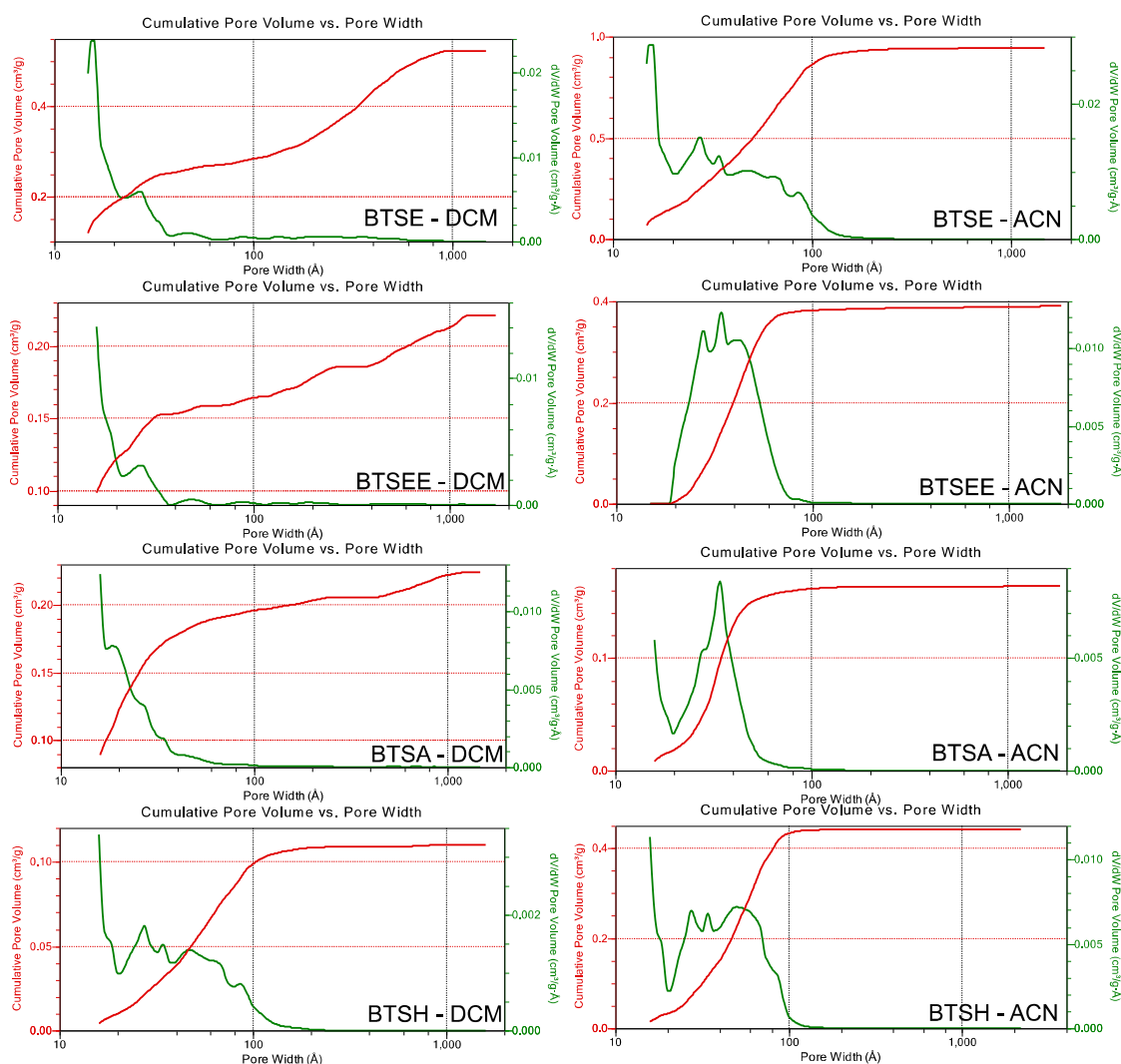
Figure 3. Density functional theory (DFT) method pore size distributions and cumulative pore volume from Brunauer–Emmet–Teller (BET) method measurement for Me-BTSE, Me-BTSEE, Me-BTSA and Me-BTSH in both DCM and ACN.
