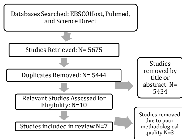
Figure 1. Search Diagram
