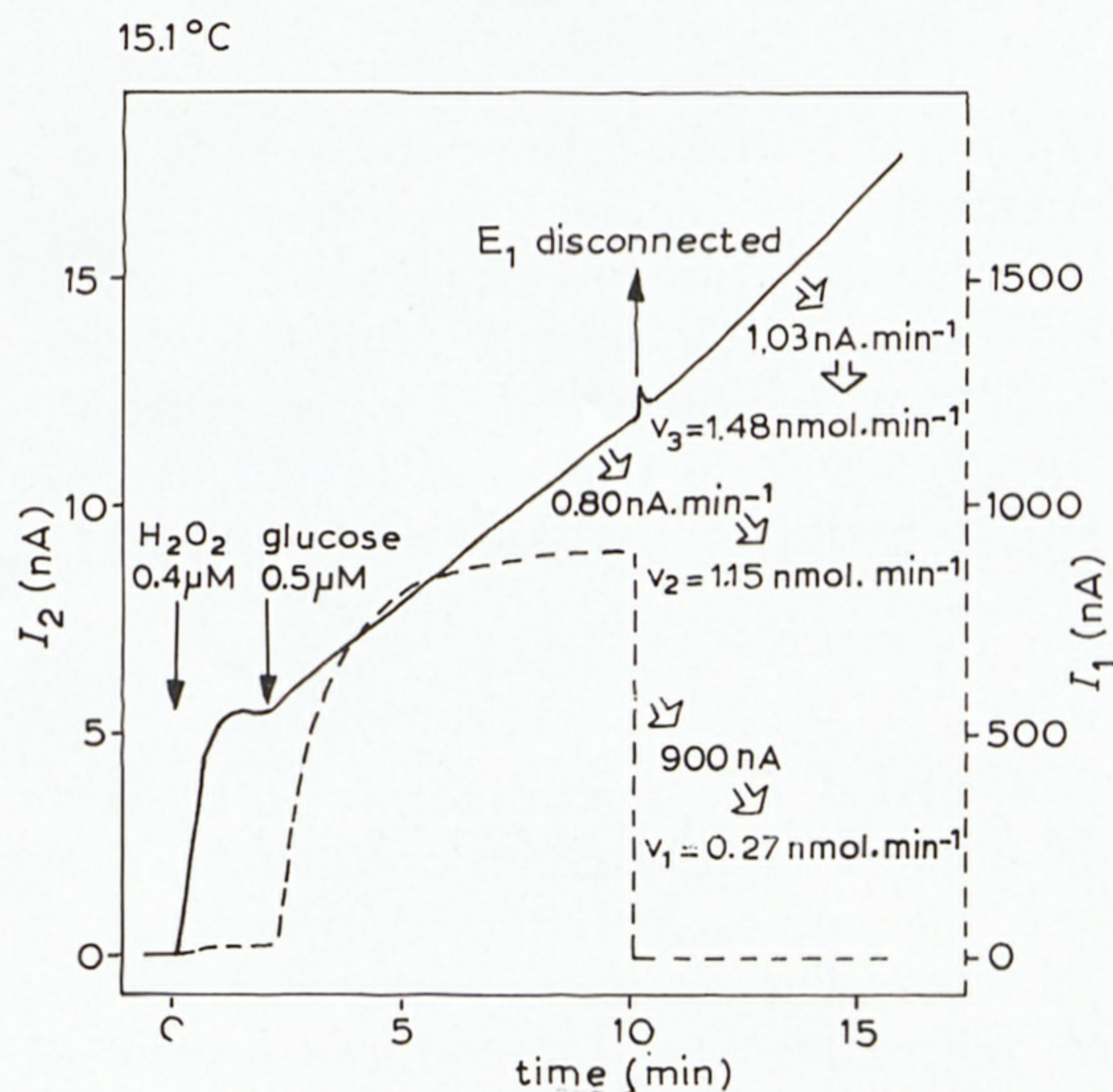
Fig. 4. Determination of hydrogen peroxide fluxes. Successive addition of 50 \mu\text{l} 0.16 \text{ mM} hydrogen peroxide and 100 \mu\text{l} 0.1 \text{ M} glucose solution into 20 \text{ ml} acetate buffer. Electrode E_1 , initially anodically polarized as electrode E_2 , is disconnected at the end of the experiment. Note the different ordinates used for each electrode.
