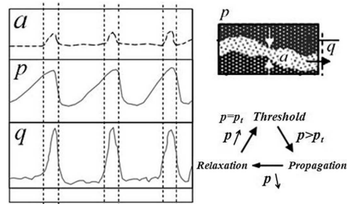
Fig. 6 The changes of pressure ( p ), flow rate ( q ) and pathway aperture ( a ) during the intermittent flow process (Alkan et al., 2008)
