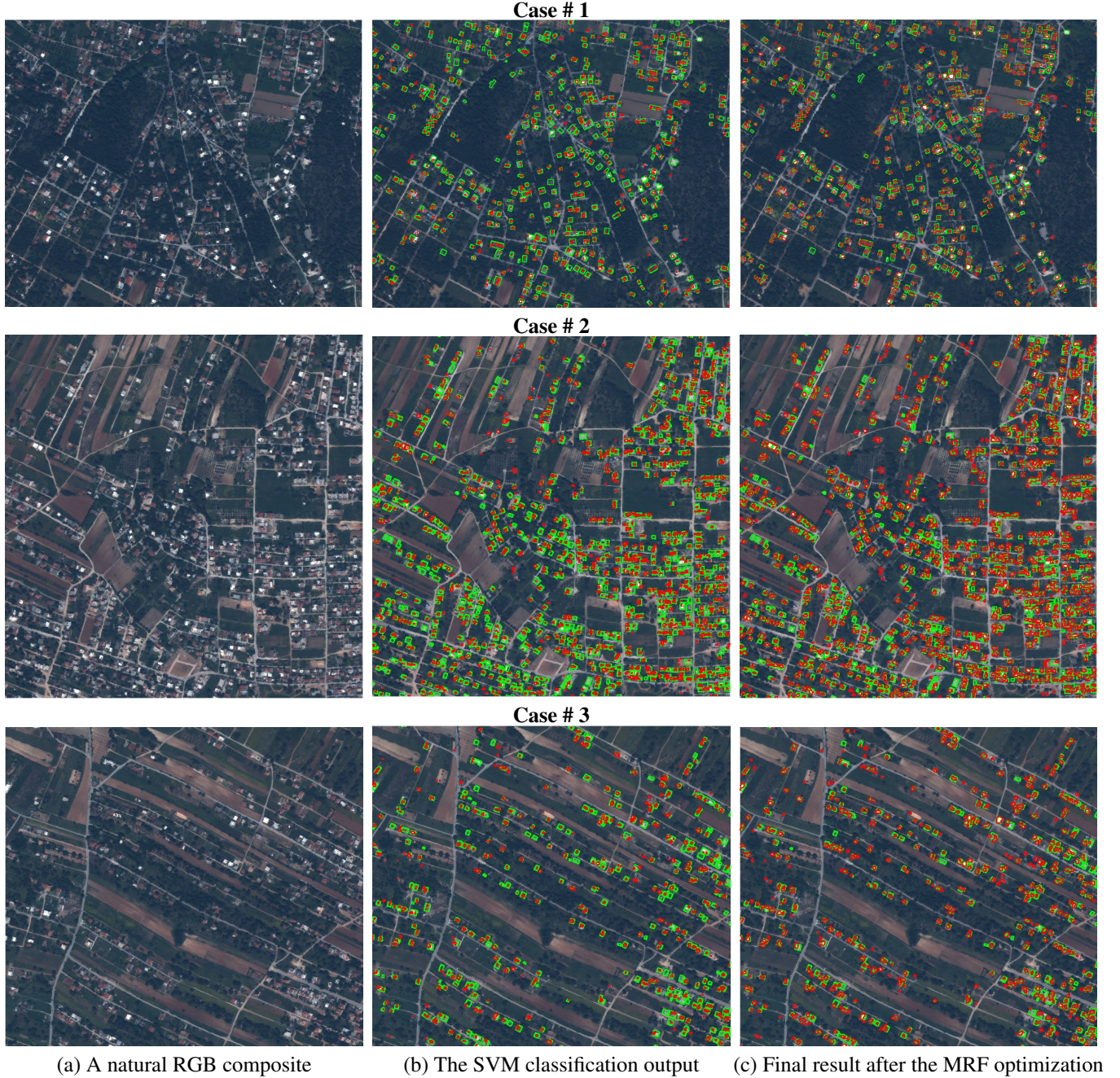
Fig. 2. Building detection on very high resolution multispectral data. The ground truth data are shown with a green color, while the detected buildings with a red one.
