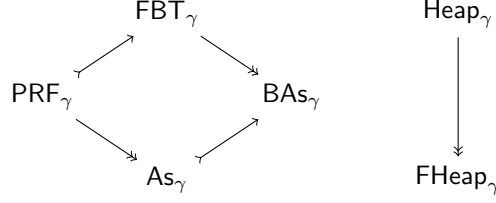
FIGURE 1. Diagram of PROs where arrows \succrightarrow (resp. \rightarrow ) are injective (resp. surjective) PRO morphisms. The parameter \gamma is a positive integer. When \gamma = 0 , \text{PRF}_0 = \text{As}_0 = \text{Heap}_0 = \text{FHeap}_0 and \text{FBT}_0 = \text{BAs}_0 .
