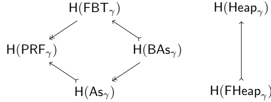
FIGURE 2. Diagram of combinatorial Hopf algebras where arrows \succrightarrow (resp. \rightarrow ) are injective (resp. surjective) PRO morphisms. The parameter \gamma is a positive integer. When \gamma = 0 , \text{H}(\text{PRF}_0) = \text{H}(\text{As}_0) = \text{H}(\text{Heap}_0) = \text{H}(\text{FHeap}_0) and \text{H}(\text{FBT}_0) = \text{H}(\text{BAs}_0) .
