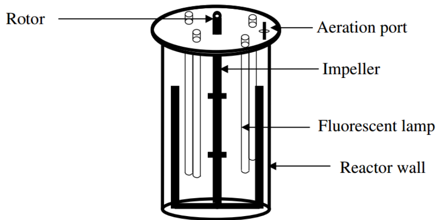
Figure 6. Internally-illuminated photobioreactor (Ugwu et al., 2008)
