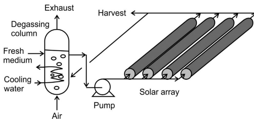
Figure 3. A tubular photobioreactor with parallel run horizontal tubes (Bahadar and Bilal Khan, 2013)
