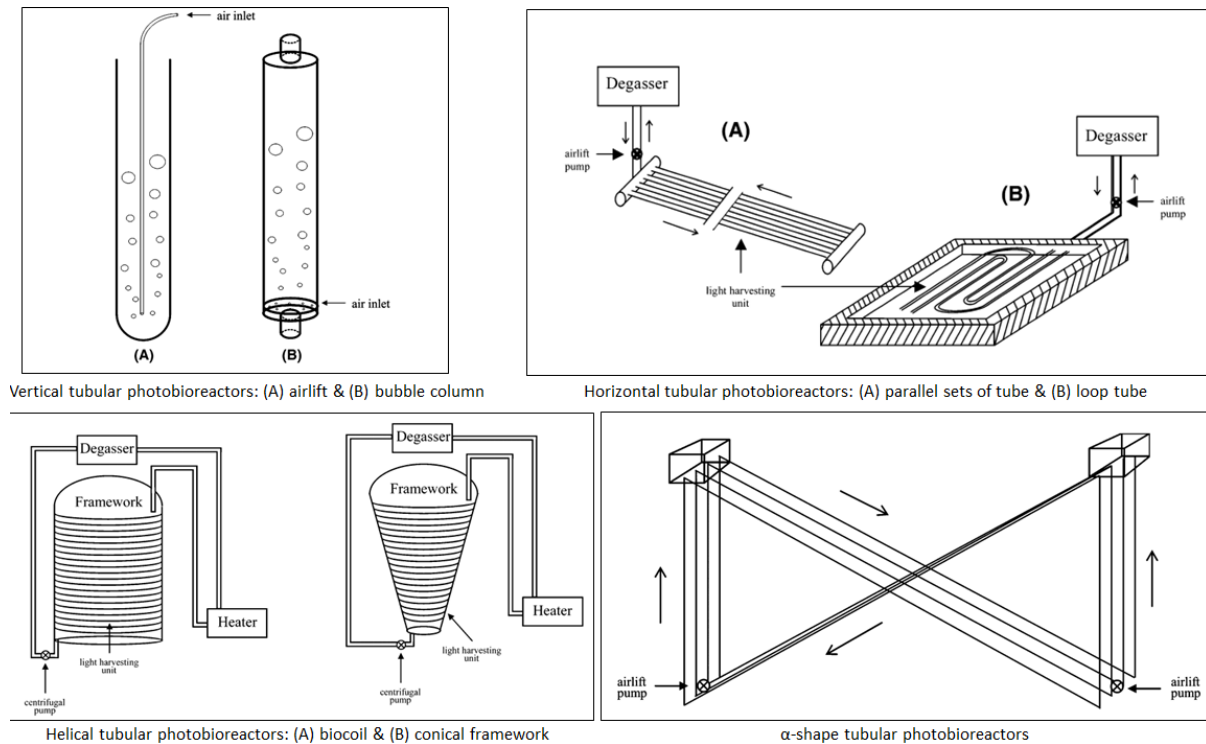
Figure 4. Types of tubular photobioreactors [Adapted from Carvalho et al., (2006)]
