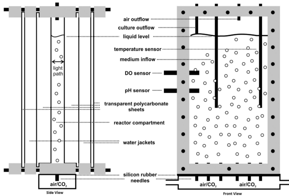
Figure 5. Front and side views of flat photobioreactor (Bahadar and Bilal Khan, 2013)
