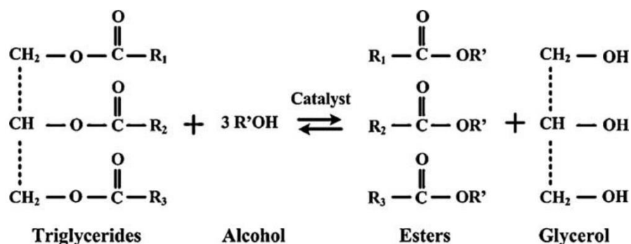
Figure 13. Biodiesel production through transesterification of triglycerides (Mata et al., 2010)
