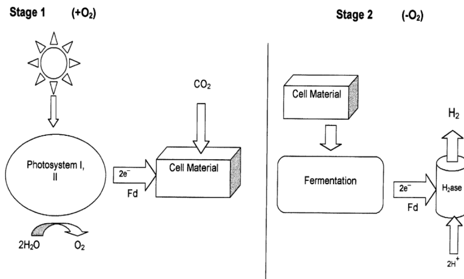
Figure 9. Indirect biophotolysis (Hallenbeck and Benemann, 2002)
