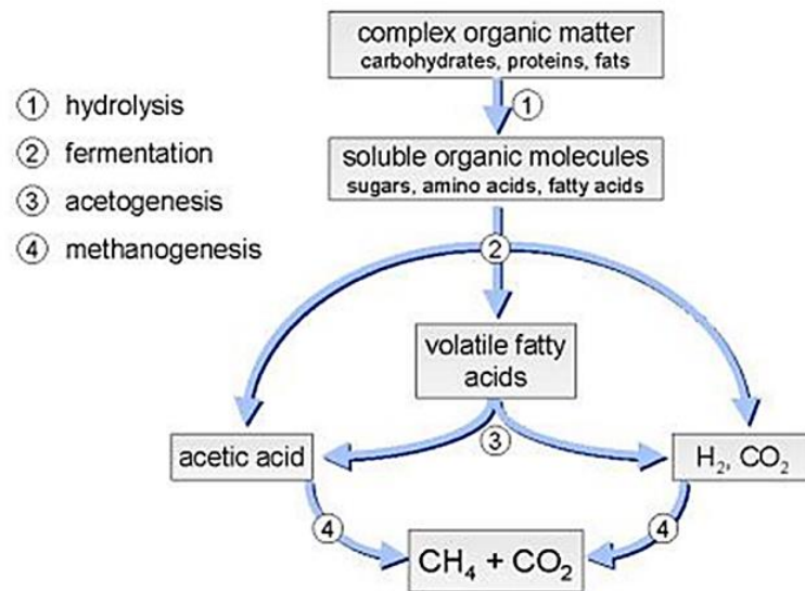
Figure 11. Biomethane production in an anaerobic digestion process (Diltz and Pullammanappallil, 2013)
