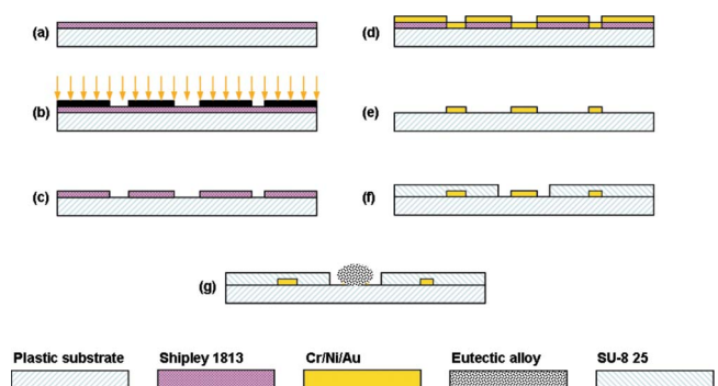
FIG. 4. (Color online) (a) Shipley 1813 (1.3 \mu\text{m} ) is deposited using PET-compatible low temperature processing. (b) Karl Suss MA6 contact aligner is used to expose photoresist to ultraviolet light. (c) LDD-26W developer is used to remove photoresist for subsequent metallization. (d) Cr/Ni/Au (5/150/100 nm) is deposited with electron beam evaporator. (e) Lift-off in acetone defines metal traces, pads, and antenna. (f) SU-8 passivation layer is applied and patterned to define solder bump regions. (g) Eutectic alloy is selectively deposited on exposed metal through liquid metal dip.
