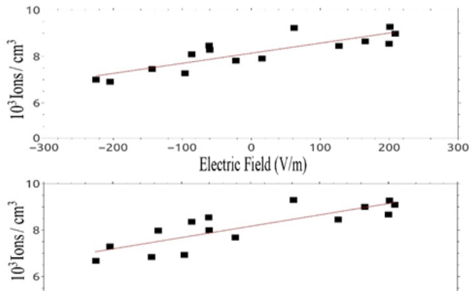
Fig. 9. Concentrations of the Atmospheric ions versus local atmospheric electric field. Top: negative ions, bottom positive ions.
