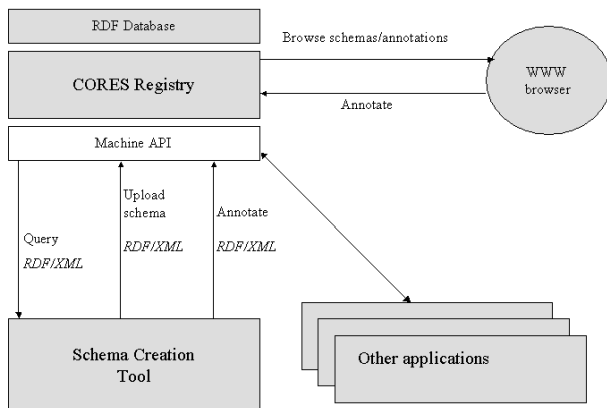
Figure 2: The registry architecture
