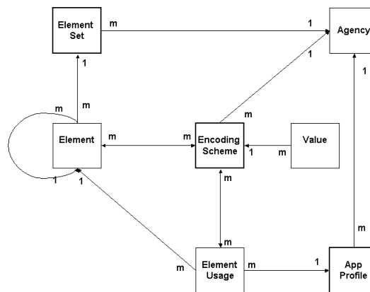
Figure 1: The base registry data model
