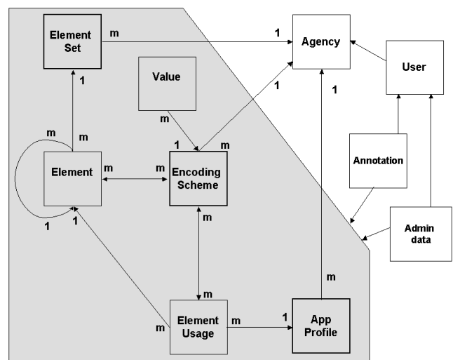
Figure 3: The extended registry data model
