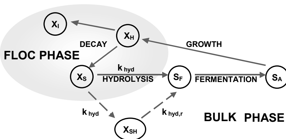
Figure 2. Scheme of the ASM2d, in continuous lines, and the modification proposed in the hydrolysis process, in dashed lines. X_I : Inert particulate substrate; X_H : Heterotrophic organisms; X_S : Particulate substrate; X_{SH} : rapidly hydrolysable substrate; S_F : Fermentable substrate; S_A : Fermentation product; K_{hyd} : First Hydrolysis stage; K_{hyd,r} : Second Hydrolysis stage.
