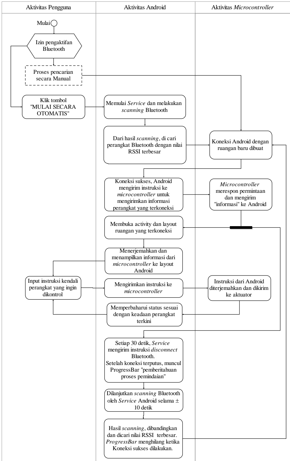
Gambar 2 Activity diagram keseluruhan system
