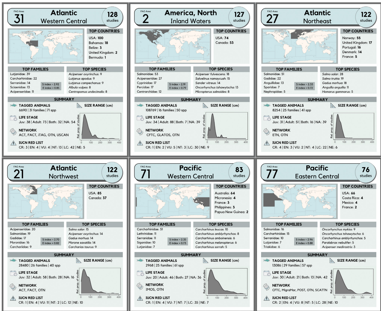
Figure 4. Acoustic telemetry (AT) study statistics for FAO major fishing areas. Summaries of study and species information are listed for each FAO area (n = 14) with more than 20 studies conducted between 2010 and 2019. All values were based on emerging trends (2010–2019) from ecology studies only. Shannon-Weaver diversity (S index) and evenness (E index) indices are based on the number of families studied and provide additional context into the composition of different focal families in AT studies. 'Tagged animals' refers to the total number of tagged individuals, families, and species inclusive of all animal groups. Life stage represents the number of studies that tagged juveniles, adults, both juveniles and adults, or it was not indicated. Where life stage was not identified in a study, it was estimated, if possible, based on the size range in the study relative to size at maturity stated on Fishbase or Sealfibase. Network terms (see Glossary) indicate established AT networks that exist (or have existed) in that area. International Union for Conservation of Nature (IUCN) Red List values represent the number of species in each designation ( https://www.iucnredlist.org/ ). Size range illustrates the distribution of the mean size of individuals tagged in each study, where stated, shown as a relative proportion of all studies in the region. Abbreviation: FAO, Food and Agriculture Organization.
