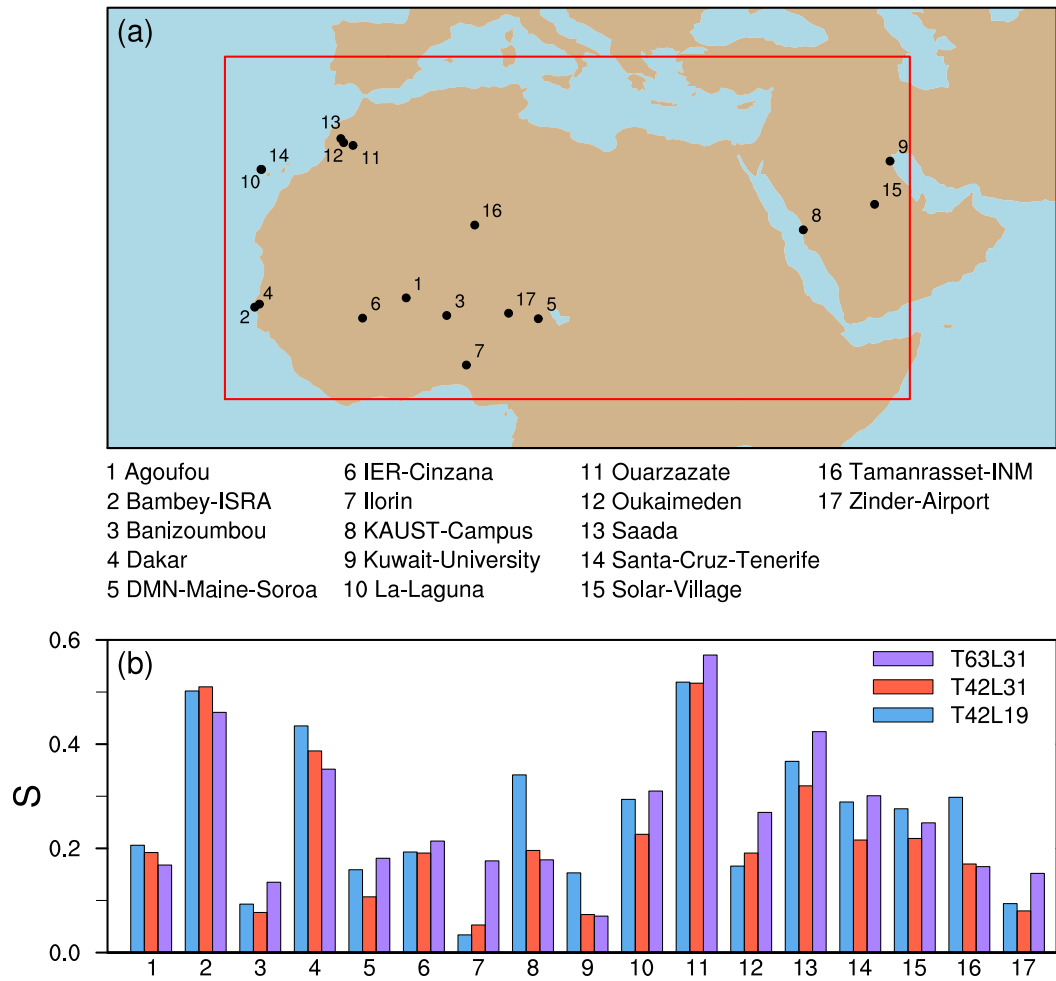
Figure A.3: As in Fig. 4.2, but comparing model results for the three different model resolutions (T42L19 in blue, T42L31 in red, T63L31 in purple). As shown in Beer et al. (2020, Fig.S6). See Sect. 4.1.2 for details.
