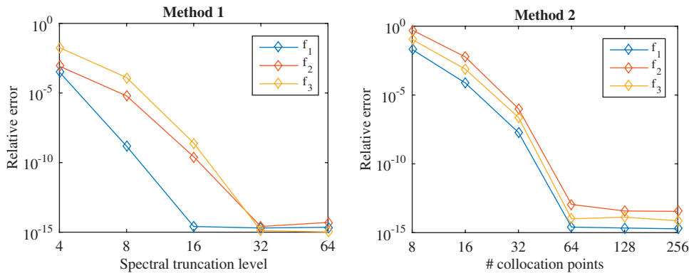
FIG. 2. Relative errors for M1 and M2 based on use of (9.1) as a consistency check.
