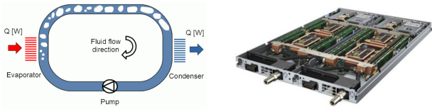
Figure 4. Schematic of the two-phase cooling system (left) and its embedding in a server (right).
