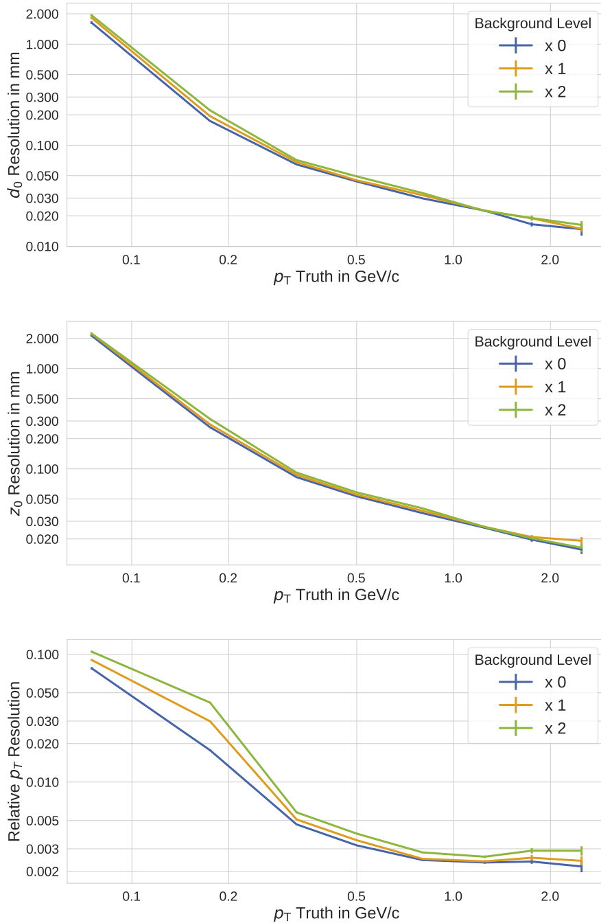
Figure 15: Resolutions for typical simulated \Upsilon(4S) events with different levels of beam-induced background. As most of the simulated final state particles are pions, only the results of this fit hypothesis are shown.
