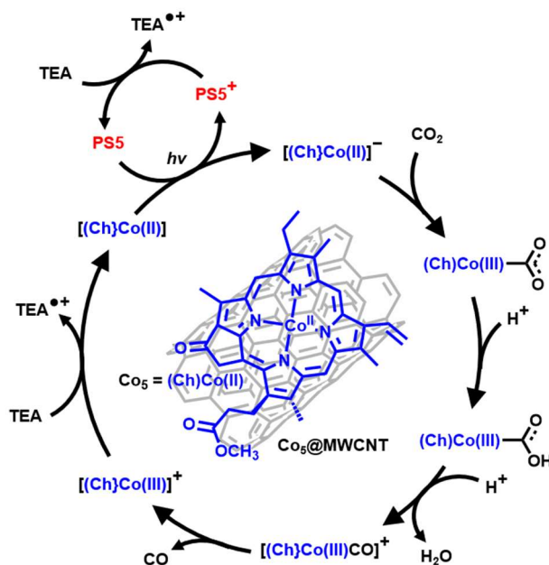
Fig. 13. Proposed mechanism for the hybrid system \text{Co}_5\text{@MWCNT} with only the path leading to CO displayed. Adapted from [54].
