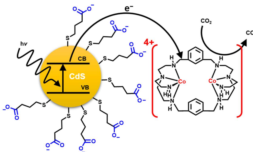
Fig. 15. Illustration of the hybrid system Co2@CdS held together by electrostatic interactions. Adapted from [56].
