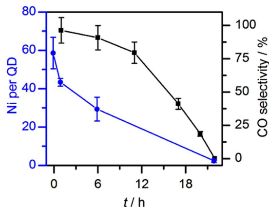
Fig. 14. Changes in product selectivity and catalyst loading over time for Ni4@CdS . Reprinted with permission from M. F. Keuhnel et al. J. Am. Chem. Soc. 139 (2017) 7217-7223. Copyright 2017 American Chemical Society. [55]
