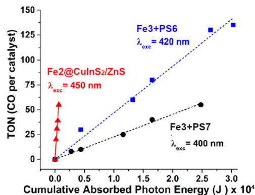
Fig. 16. Measurement of sensitization efficiency and comparison between Fe2@CuInS 2 /ZnS (red), PS6 - (blue) and PS7 -sensitized (black) Fe3 catalyst. Adapted with permission from S. Lian et al. J. Am. Chem. Soc. 139 (2017) 8931-8938. Copyright 2017 American Chemical Society.[58].
