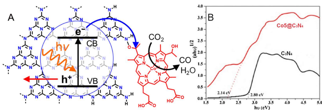
Fig. 9. A. Proposed mechanism for CO 2 reduction with the Co5@C 3 N 4 system. B. Plot of Kubelka-Munk function vs. exciting light energy. Bandgap energy values for Co5@C 3 N 4 and C 3 N 4 extrapolated from the absorption edges. Reproduced from [46].
