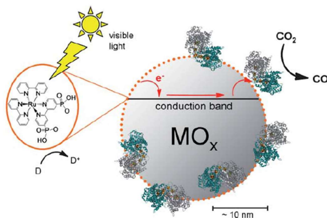
Fig. 19. Illustration of \text{CO}_2 reduction at the CODH- and PS1 -modified \text{TiO}_2 surface driven by visible light. D: MES. Reproduced from [64].
