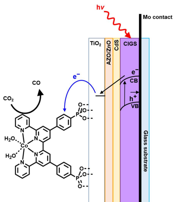
Fig. 24. A diagram of the CIGS photocathode functionalized for PEC CO 2 reduction with a phosphonated analogue of the Co2 catalyst. Adapted from [76].
