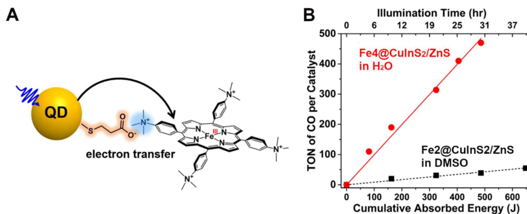
Fig. 17. a. Schematic representation of electron transfer and electrostatic interactions in the \text{Fe}_4@\text{CuInS}_2/\text{ZnS} hybrid system; b. comparison of sensitization efficiency between the \text{Fe}_4 - (red) and \text{Fe}_2 -containing (black) systems. Adapted with permission from S. Lian et al. ACS Nano 12 (2018) 568-575. Copyright 2018 American Chemical Society.[59].
