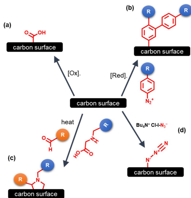
Fig. 5. Examples of commonly used methods to covalently bind anchoring groups onto carbon surfaces: (a) oxidation to introduce C-O functionalities; (b) reduction of diazonium salts; (c) 1,3-dipolar cycloaddition of azomethine ylides to form pyrrolidine units; (d) introduction of azide groups. Adapted from [4].
