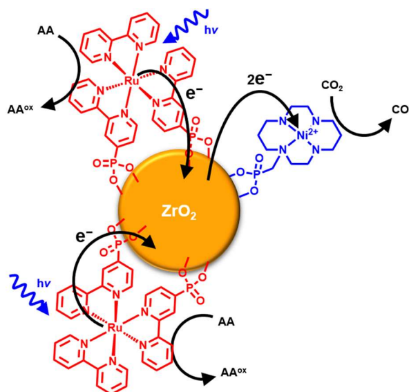
Fig. 20. Nickel catalyst and ruthenium photosensitizers co-immobilized on a \text{ZrO}_2 particle to form \text{Ni5@ZrO}_2 hybrid system. Adapted from [65].
