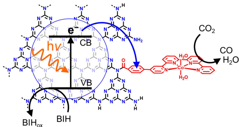
Fig. 11. Illustration of the Co 2 @C 3 N 4 hybrid system. Adapted from [52].
