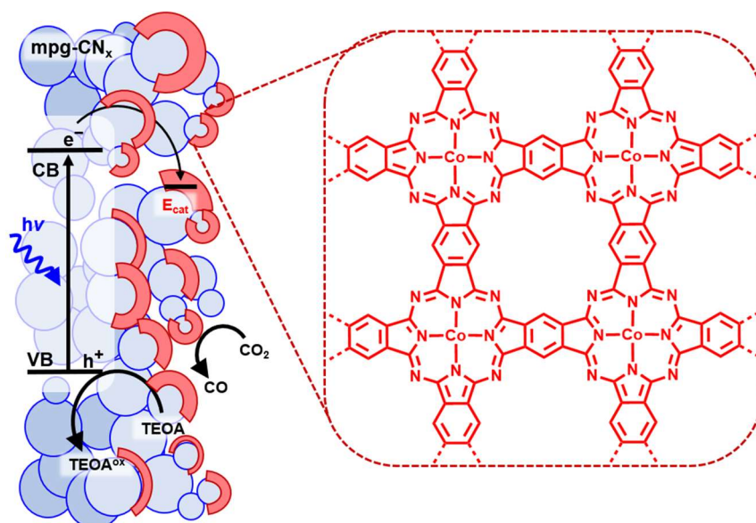
Fig. 10. Illustration of the photocatalytic \text{CO}_2 reduction achieved using Co3@C 3 N 4 hybrid system. Adapted from [51].
