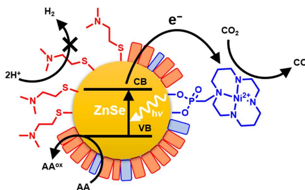
Fig. 18. Schematic representation of the hybrid system Ni2@ZnSe with the QD particle partially capped by MEDA. AA: ascorbic acid. Adapted from [60].
