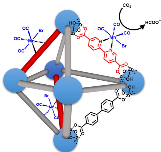
Fig. 21. Representation of the Mn1@UiO-67 hybrid structure catalysing \text{CO}_2 reduction after electron transfer from PS2 . The bipyridine modified bridging ligands (red) are shown coordinated to the catalyst ( Mn2 blue) and octahedral zirconium oxide corner units (light blue). Adapted from [66]
