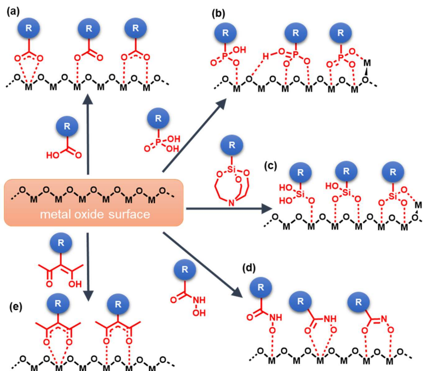
Fig. 7. Surface binding modes of different anchors onto metal oxide materials: (a) carboxylates, (b) phosphonates, (c) silatranes, (d) hydroxamates and (e) acetylacetonates. Adapted from [4].
