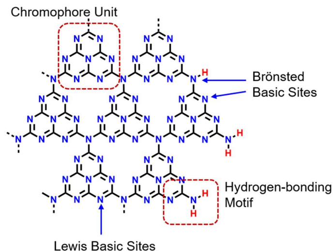
Fig. 4. Structure of tris-S-triazine, one of the possible g\text{-C}_3\text{N}_4 allotropes, indicating basic sites and hydrogen bonding motifs in the structure. Adapted from [18].
