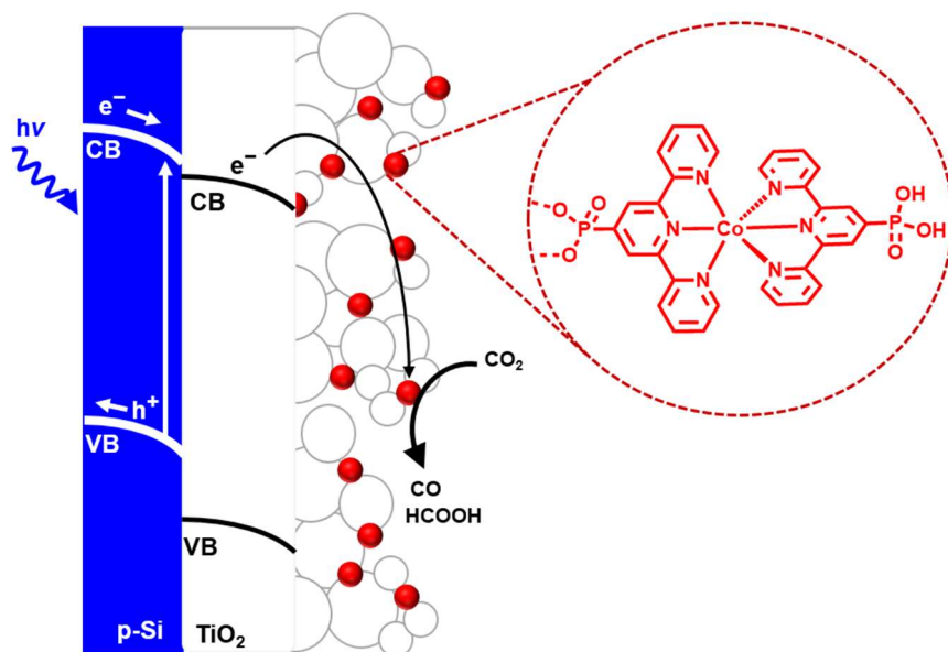
Fig. 25. Schematic representation of the hybrid system. Adapted from [77].
