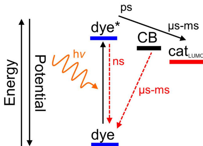
Fig. 2. Electron transfer cascade in the DSP setting. Forward transfer and recombination rates are indicated in black and red, respectively. CB: conduction band of the semiconductor. Adapted from [7].
