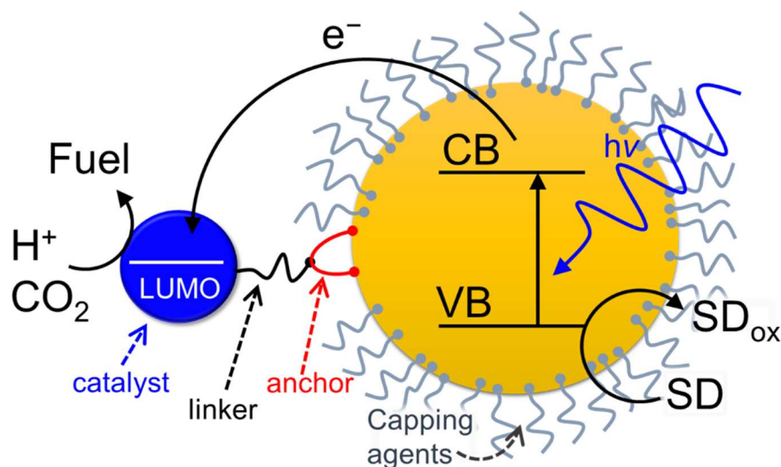
Fig. 3. Representation of CO 2 reduction with a catalyst (blue) attached to a QD (yellow) where the latter acts as a photosensitizer and is regenerated by a SD. Adapted from [8].
