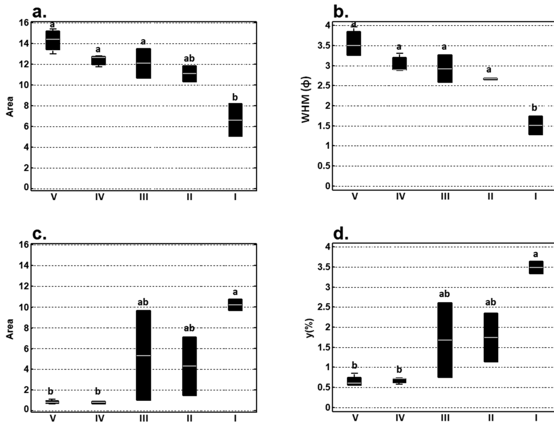
Fig. 6. Box plots for (a) Area of M_{FSI} according to deposition ( p < 0.01 ); (b) WHM of M_{FSI} according to deposition ( P < 0.01 ); (c) Area of M_C according to deposition ( p < 0.01 ); (d) y of M_C according to deposition ( P < 0.05 ).
