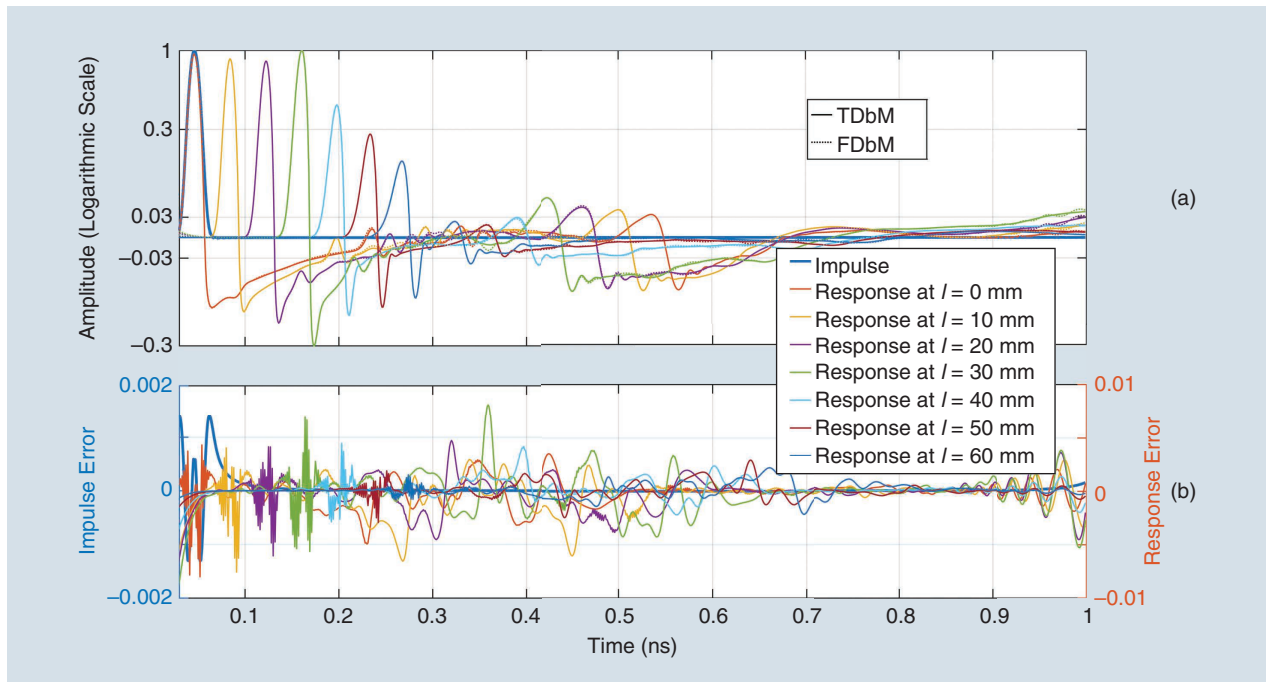
FIGURE 4. The impulse and responses pairs with (a) TDdBm and FDdBm and (b) the corresponding errors.
