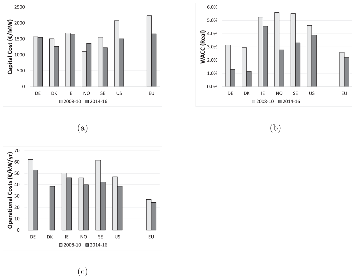
Fig. 4. Cost and financing trends in participating countries (weighted averages) (a) unit capital cost (CapEx); (b) after-tax real weighted average cost of capital (WACC); and (c) unit operational cost (OpEx). (Notes: 2009, 2014 DE data, 2009, 2010 DK and 2009, 2010 NO data unavailable for (a). 2009, 2010 NO data unavailable for (b); 2009 DE, 2008–10 DK data and 2009, 2010 NO data unavailable for (c)).
