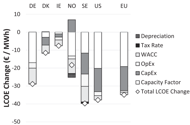
Fig. 6. Contribution of input variables to changes in average national LCOEs for 2008–10 and 2014–16.
