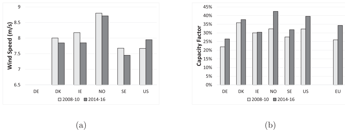
Fig. 3. Site trends in participating countries (weighted averages) (a) wind speeds adjusted to 100 m elevation; (b) capacity factors. (Notes: no DE data available for (a); no EU data available for (a); 2009, 2010 NO data unavailable for (a) and (b)).
