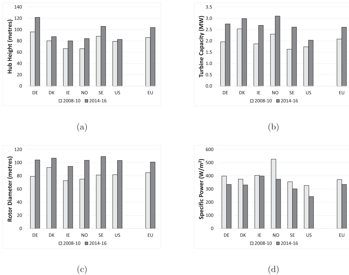
Fig. 2. Technology trends in participating countries (capacity-weighted averages) shown for the periods 2008–2010 and 2014–16: (a) hub height; (b) turbine nameplate capacity; (c) rotor diameter (d) turbine specific power. (Notes: 2009, 2010 NO data unavailable for (a)–(c); 2016 EU data unavailable for (a)).
