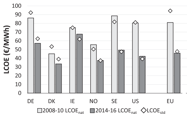
Fig. 5. Levelized costs of energy results: 2008–10 and 2014–16 average LCOE_{nat} and LCOE_{std} .
