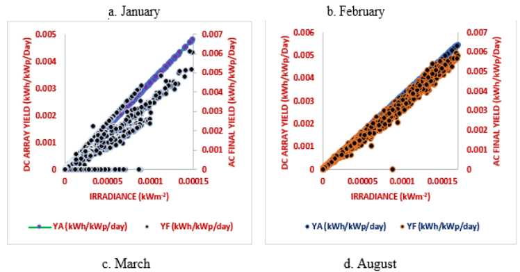
Figure 8: Quarter-Hourly data for AC Final yield and DC Array yield.
