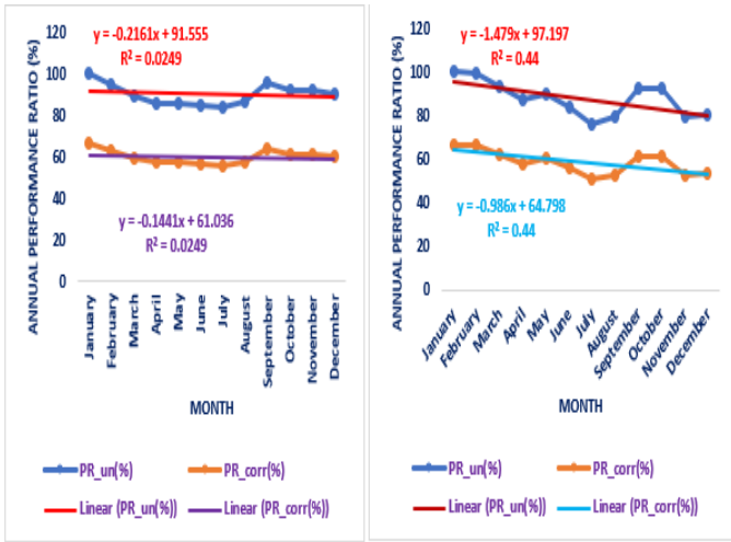
Figure 15: Annual System PR for 2018
