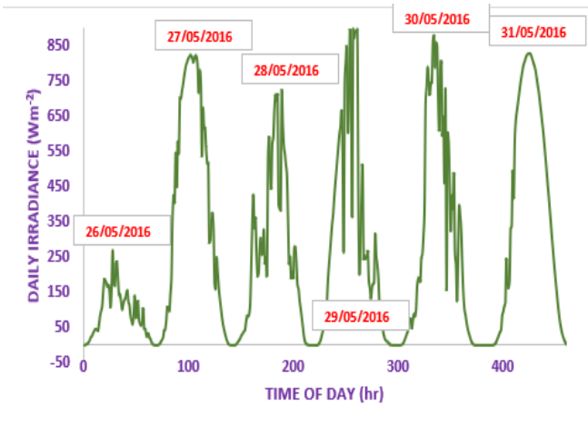
Figure 10: Measured solar irradiance profiles for each day in May 2016.
