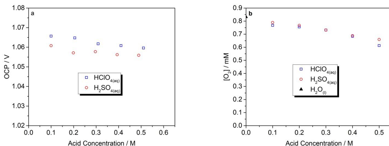
Figure 4. (a) The measured OCP of a Pt/C (JM) GDE with different acid concentrations. (b) The measured [O 2 ] in the electrolytes through use of a Clark cell.
