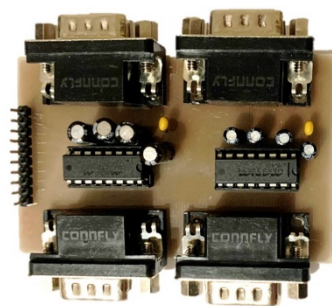
Figure 7: 4x RS232 - UART interface module
