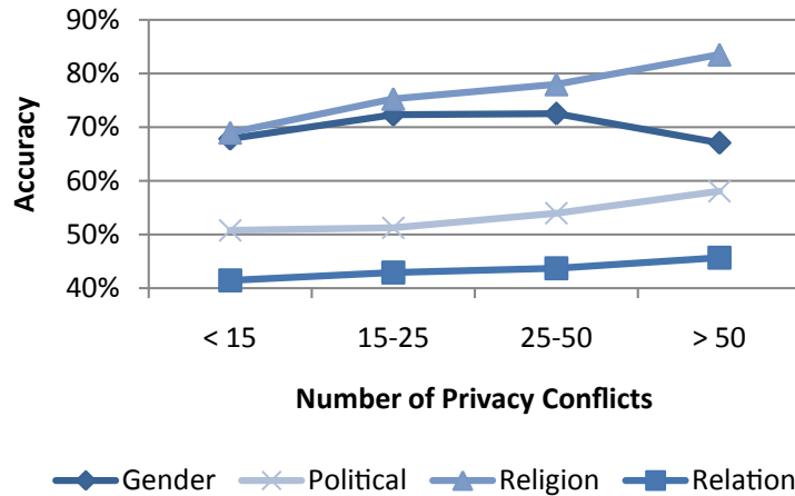
Figure 6.2: Accuracy of the friend classifier grows roughly linearly as a function of the number of privacy conflicts.
