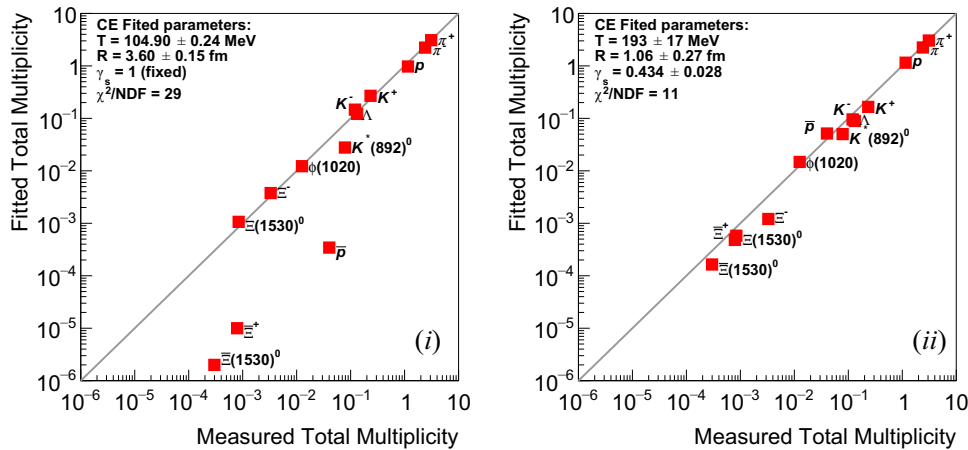
Fig. 11 Mean multiplicities of \pi^+ , \pi^- , K^+ , K^- , p , \bar{p} , K^*(892)^0 , \Lambda , \phi(1020) , \Xi^- , \bar{\Xi}^+ , \Xi(1530)^0 and \bar{\Xi}(1530)^0 produced in p+p interactions at 158 GeV/c [3, 4, 12, 17–20] measured by NA61/SHINE are com-
