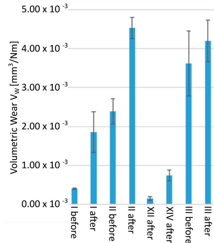
Figure 7. Volumetric loss V_w of the tested polymers.
