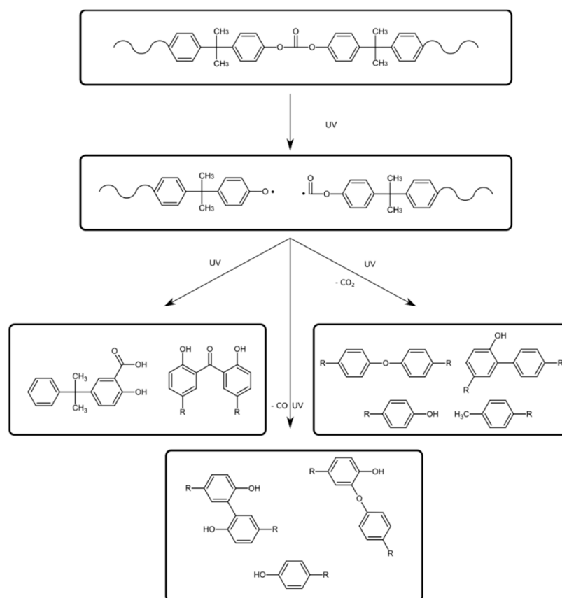
Figure 2. Photodegradation of polycarbonate.
