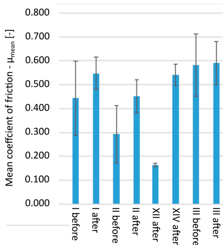
Figure 8. Changes in the stabilized coefficient of friction \mu of the tested materials.
