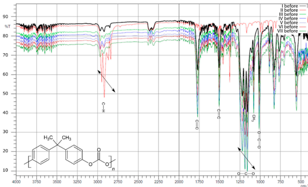
Figure 3. Compilation of IR spectra before aging for samples I, II, III, IV, V, VI, and VII.
