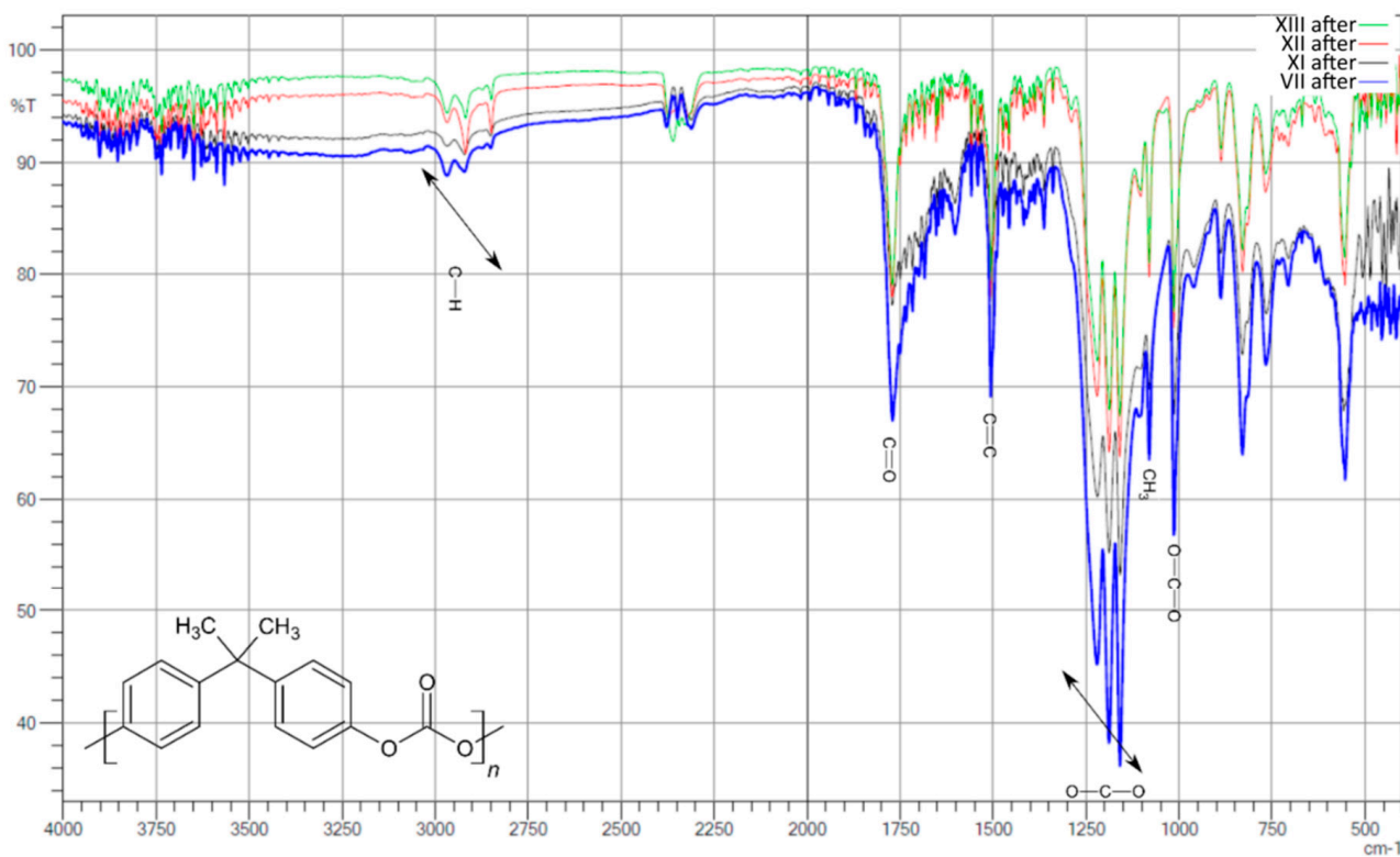
Figure 6. Compilation of IR spectra after aging for samples XIII, XII, XI, and VII.
