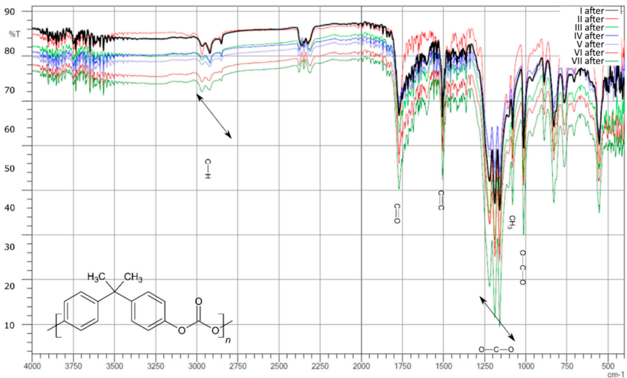
Figure 4. Compilation of IR spectra after aging for samples I, II, III, IV, V, VI, and VII.
