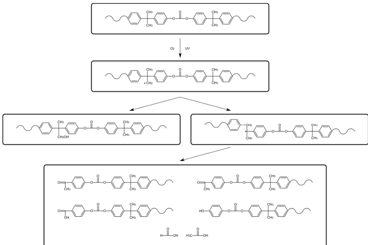
Figure 1. Photo-oxidative degradation of polycarbonate.
