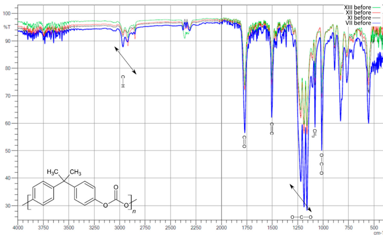
Figure 5. Compilation of IR spectra before aging for samples XIII, XII, XI, and VII.
