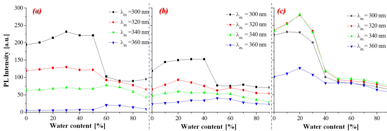
Figure 6. Changes in the PL intensity versus the water content ( f_w ) in a binary mixture of \text{CH}_3\text{CN}/\text{H}_2\text{O} with an increasing water content ( f_w = 0\%, 10\%, 20\%, 30\%, 40\%, 50\%, 60\%, 70\%, 80\%, 90\%, v/v ) at different excitation wavelengths ( \lambda_{\text{ex}} : 300, 320, 340, 360 nm) for: (a) 4, (b) 5, (c) 6 (cf. Figure S12).
