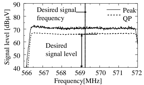
(b) Spectrum of digital TV
