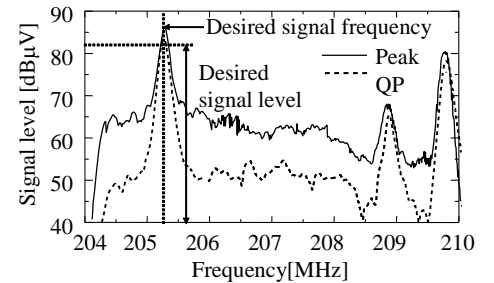
(a) Spectrum of analogue TV
