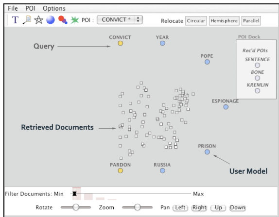
Figure 1: Adaptive VIBE Visualization (in Hemisphere layout)
