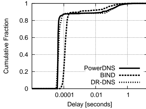
Figure 3.4: Amount of delay required to process requests.
