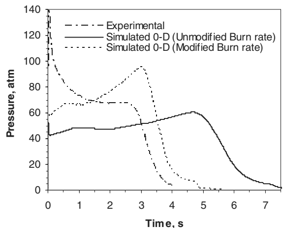
Fig. 10 0-D pressure: NAWC motor no. 6.
