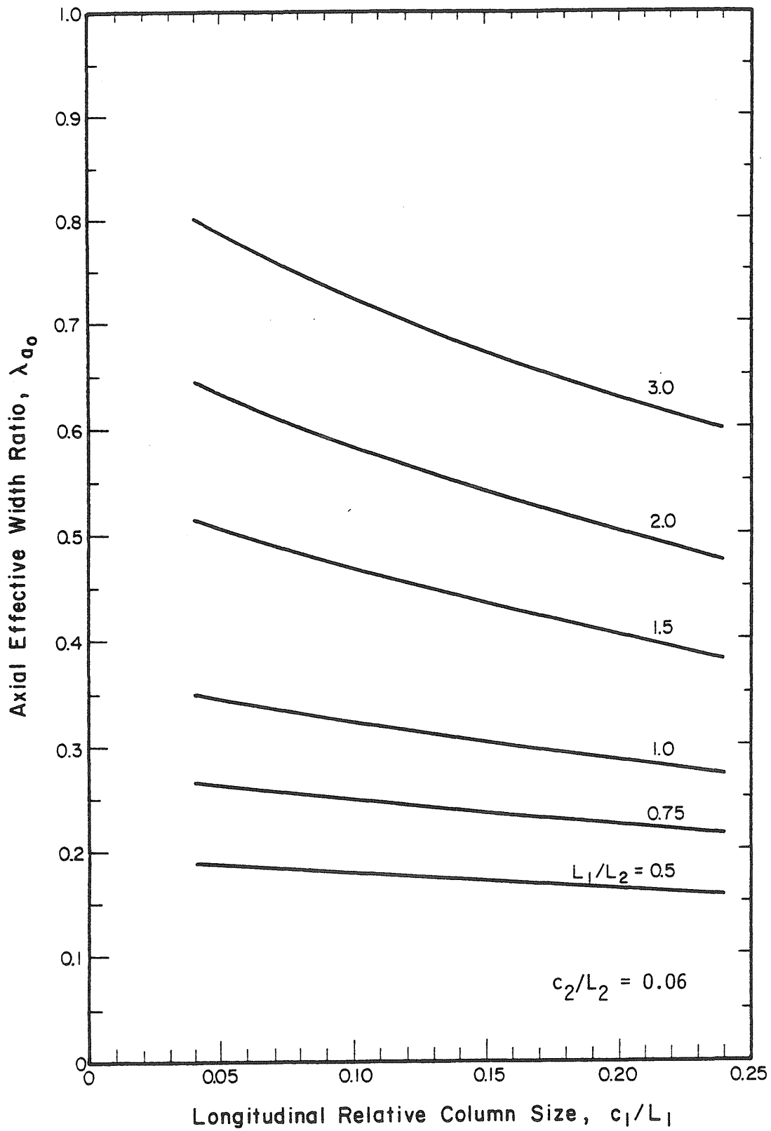
Fig. 3.3 Axial Effective Width Ratios
