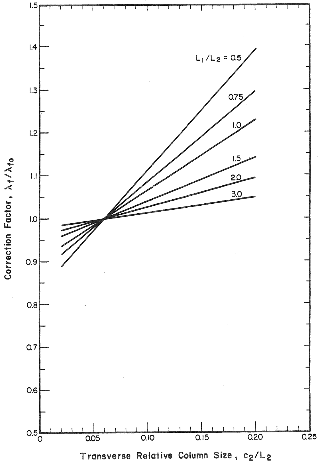
Fig. 3.2 Correction Factors for Flexural Effective Width Ratios
