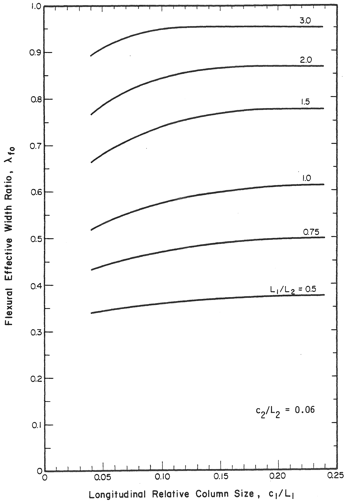
Fig. 3.1 Flexural Effective Width Ratios
