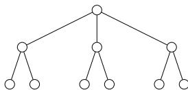
Figure 2: The graph H_3 .
