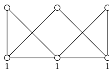
Figure 2. A graph G with \gamma_{tr}(G) = \gamma(G) + 1 .
