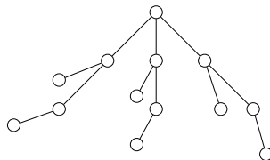
Figure 3: The structure of the tree R_3 .
