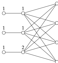
Figure 5. The graph G_{3,4} .
